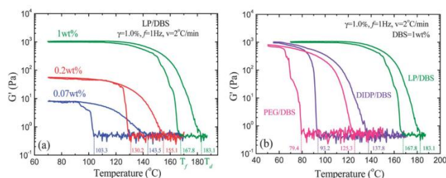
Fig. 11. The dependence of G' on the temperature at a heating and cooling rate of 2\text{ }^\circ\text{C min}^{-1} : (left) LP-DBS gels containing 0.07 wt%, 0.2 wt% and 1 wt% DBS. (right) 1 wt% DBS in LP-DBS, DIDP-DBS and PEG-DBS gel systems, respectively. The strain amplitude and frequency are 1.0% and 1 Hz. Figure reproduced from reference 49 with permission from The Royal Society of Chemistry.
