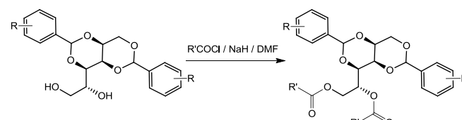
Scheme 4. Esterification of the free hydroxyl groups of DBS and derivatives by acylation.
