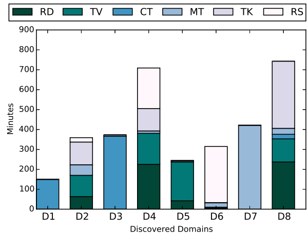
Figure 2: Amount of data for each discovered domain ( K = 8 ) from the labelled domains using a codebook size of 2,048
