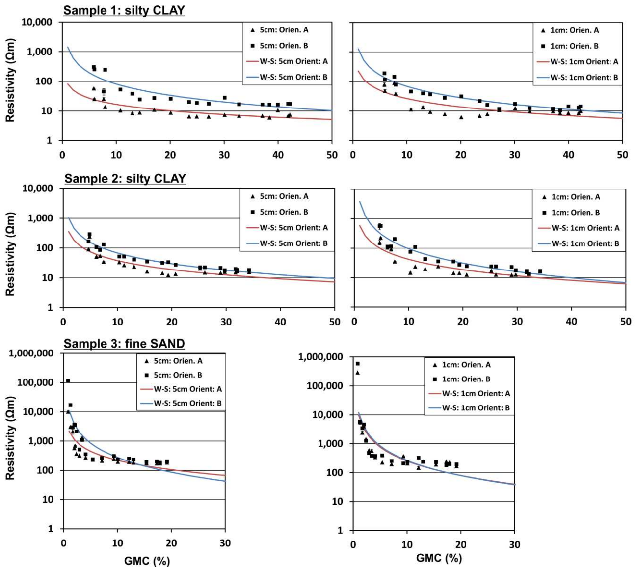
Figure 5. Electrical resistivity – soil moisture content relationship of earthflow deposits of the Hollin Hill landslide system. Presented are the associated Waxman-Smith models for each of the electrical measurement orientations.
