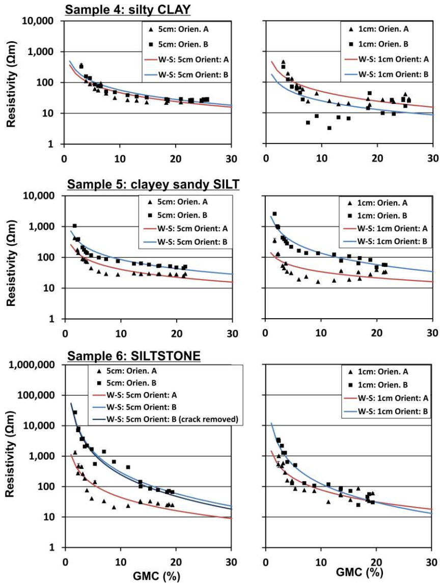
Figure 6. Electrical resistivity – soil moisture content relationship of slump deposits and in-situ material of the Hollin Hill landslide system. Presented are the associated Waxman-Smith models for each of the electrical measurement orientations.
