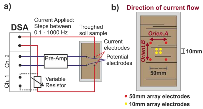
Figure 3. a) (left) Electrical circuit diagram of Digital Signal Analyser circuit board and pre-amplifier experimental setup (adapted from Ntarlagiannis et al., 2005) b) (right) Diagram of sample trough along with electrode array locations, measurement dimensions and current flow directions.
