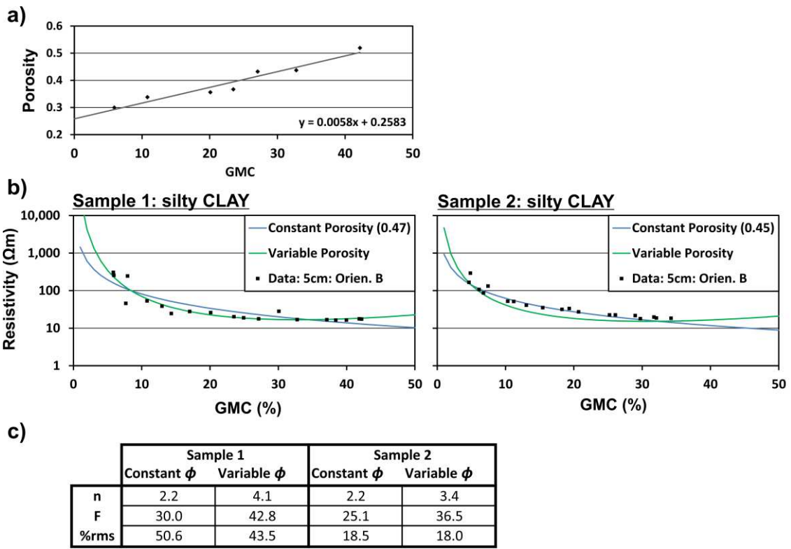
Figure 8. Comparison between Waxman-Smit models between porosity-constant and porosity-variable models.
