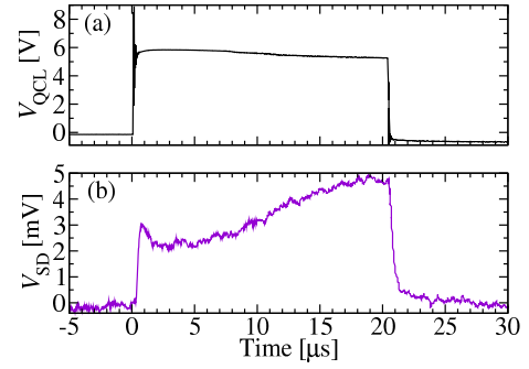
Figure 2. (a) The time-domain voltage signal measured across the 2.56-THz QCL in response to a single current pulse, corresponding to its peak emission power. (b) The corresponding baseline-corrected response of the detector.
