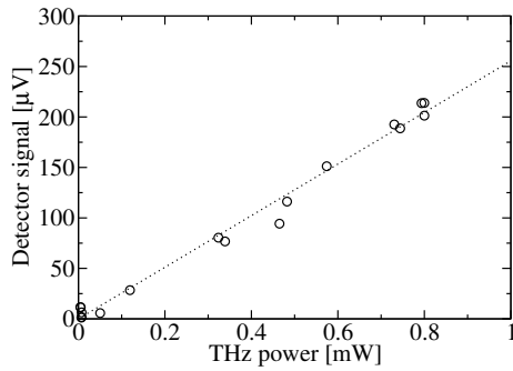
Figure 3. Time-averaged detector response at 2.2 THz as a function of the time-averaged THz QCL power.
