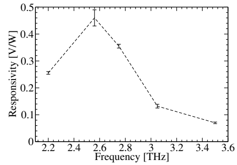
Figure 4. Detector responsivity as a function of THz frequency. The dashed line is a guide for the eye. Error bars show the fitting-uncertainty in the relationship between detector signal and power.
