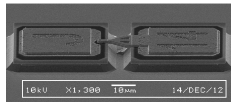
Figure 1. A scanning electron microscope image of a planar airbridged GaAs Schottky diode similar to the devices used in this work
