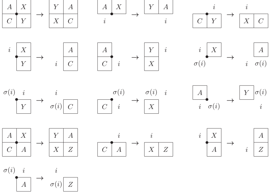
FIGURE 30. Local mutation rules for labellings
