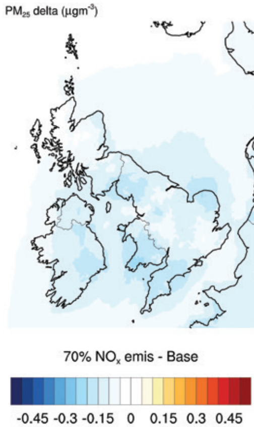
Figure 13: Change in PM 2.5 (µg m -3 ) simulated by the EMEP4UK model for 70% of UK NO x emissions (i.e. 30% emissions reduction).
