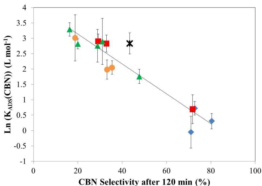
Figure 7: Fitted adsorption constant, K_{arom,CBN} plotted against CBN selectivity after 120 min for a range of solvents tested. (◆) denotes alkane solvents, (■) aromatics, (▲) primary alcohols, (●) secondary alcohols, (*) ethers. N.B.: No significant adsorption constant was found for halogenates.
