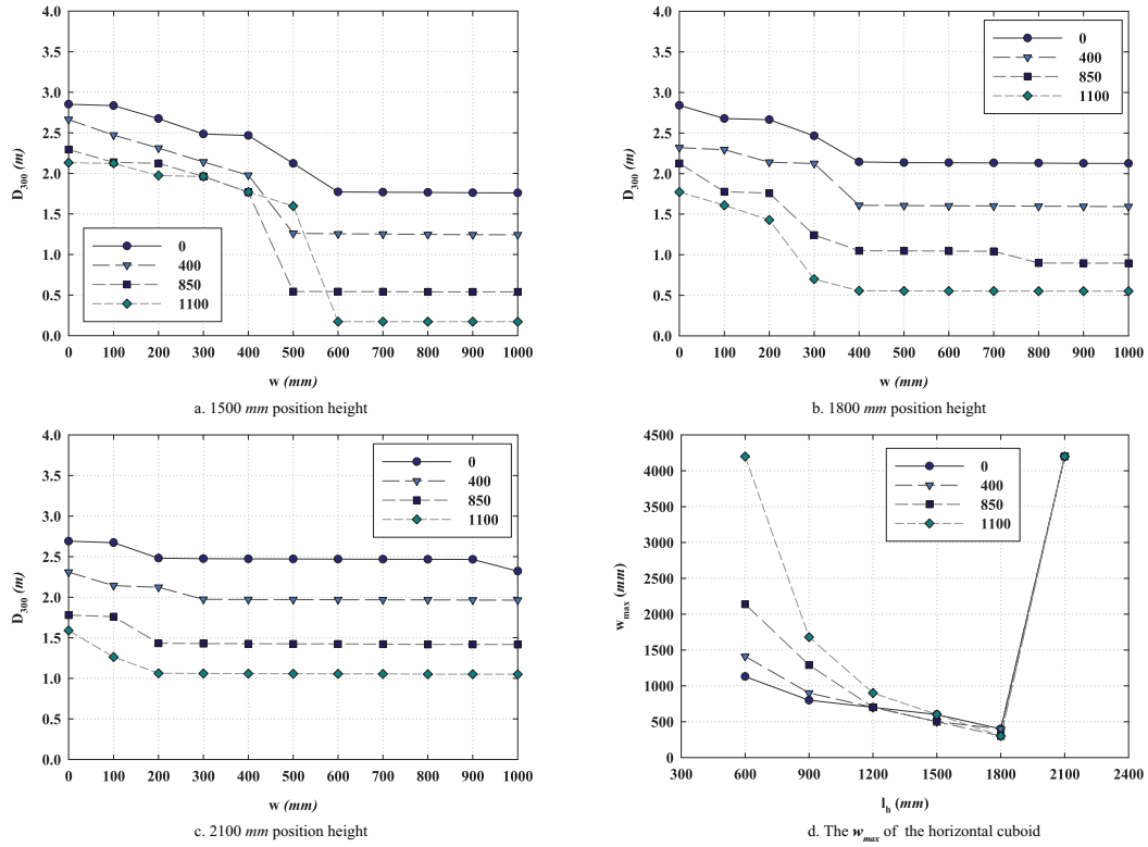
Fig. 12 D values of the horizontal cuboid with different widths at different position heights for the 300 lux illuminance contour and the w max of the horizontal cuboid for the 300 lux illuminance contour on the 850 mm high working plane
