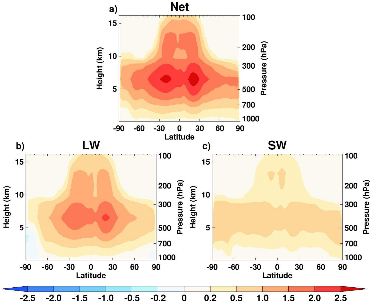
Figure S1. Annual zonal mean tropospheric ozone instantaneous radiative kernel (IRK) under all sky conditions in units of mW m -2 per ppbv for (a) net (LW+SW), (b) LW and (c) SW.
