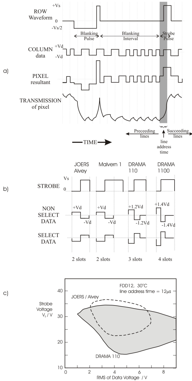
Figure 13. \tau V_{min} addressing a) Timing diagram for a row operating with the Malvern scheme [35]; b) Strobe and data waveforms for JOERS/Alvey, Malvern and DRA Multiplex Addressing (DRAMA) schemes; c) Mixture FDD12 \tau V_{min} operation with DRAMA 110 scheme [36] operating at 12 \mu s per line.
