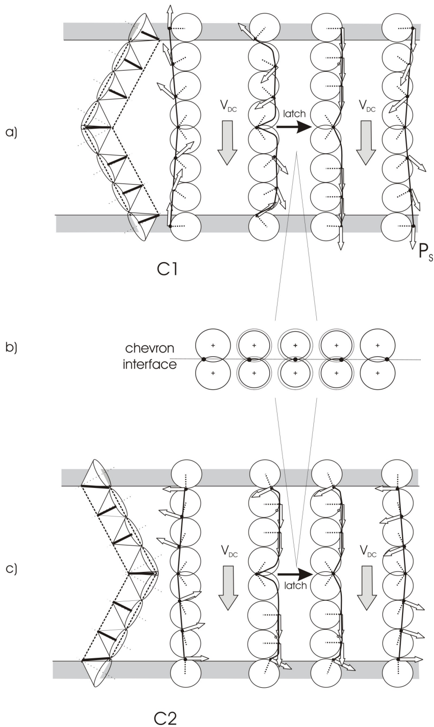
Figure 11. Ferroelectric liquid crystal latching between “up” and “down” states. a) Latching in the C1 chevron state with high pre-tilt; b) potential model for latching at the chevron interface, c) Latching in the C2 chevron state with low pre-tilt.
