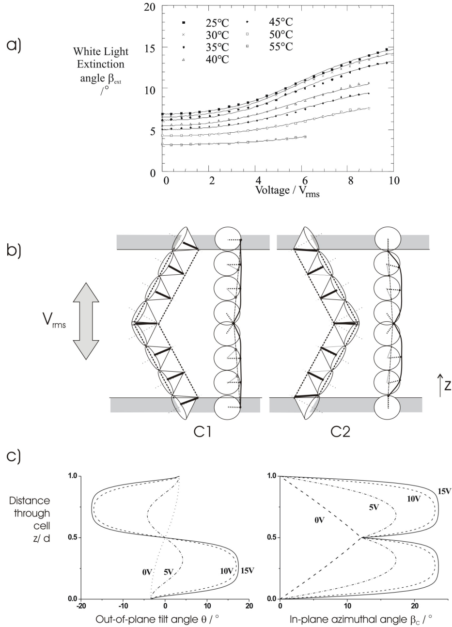
Figure 10. AC field stabilisation. a) The white light extinction angle versus applied V_{\text{rms}} for a 1.5\mu\text{m} sample of SCE8(R) in the C2 geometry at several temperatures across the smectic C range; The lines represent theoretical fits calculated using \theta_C = 55.3^\circ(1-T/T_C)^{0.32} , \delta_C = 46.2^\circ(1-T/T_C)^{0.31} , \partial\epsilon = 10.8(1-T/T_C)^{0.63} , B_1 = B_2 = 69.8\text{pN}(1-T/T_C) and T_C = 61.8^\circ\text{C} . b) The effect of an applied AC field in high surface pre-tilt C1 and low surface pre-tilt C2 geometries; c) Theoretical predictions for the tilt and azimuthal angles for the C2 geometry with applied AC field coupling to the dielectric biaxiality
