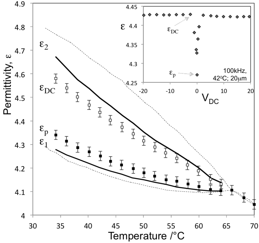
Figure 18. Perpendicular permittivities for a FLC mixture similar in composition to SCE8 measured using DC switching. Solid lines show the values obtained from extrapolation of the mean permittivity. Inset is an example of the FLC permittivity behaviour with applied DC voltage.
