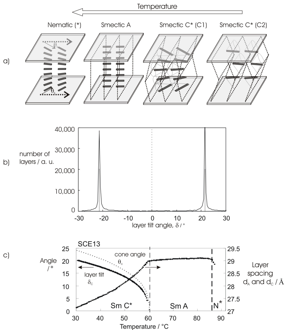
Figure 3. Formation of “chevron” layer structures on cooling a parallel-aligned planar homogenous sample through the nematic-Smectic A to Smectic C* sequence. a) Formation of C1 and C2 layer tilt; b) Smectic layer distribution at 30°C for the commercial FLC mixture SCE13 determined by X-ray diffraction; c) Temperature dependence of the layer spacing, layer tilt and optical cone angle.
