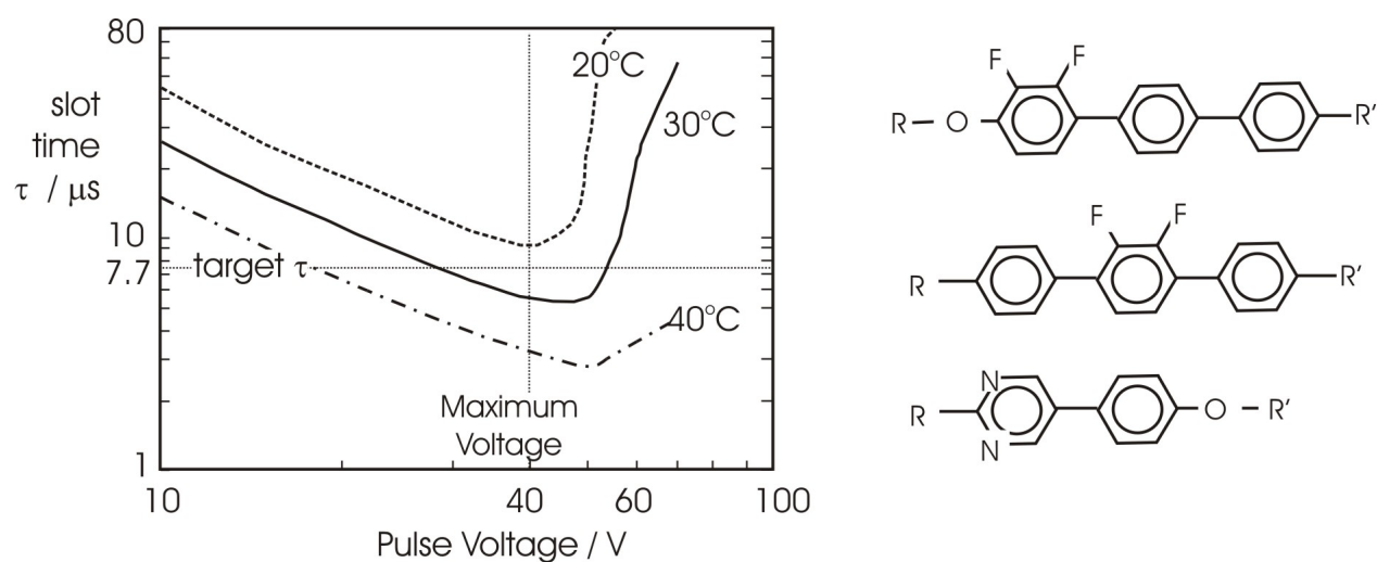
Figure 24. Low viscosity high dielectric biaxiality mixtures for use in \tau V_{\min} SSFLC [50].
