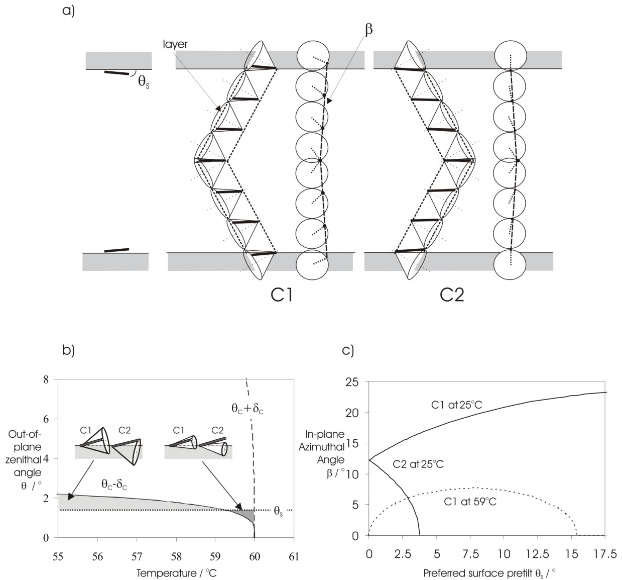
Figure 4. The relationship between surface pre-tilt and smectic C (*) layer orientation. a) Schematic of the director profiles for parallel-aligned surfaces with pretilt \theta_s in the C1 and C2 chevron arrangements; of surface pretilt on the layer and director profiles; b) Temperature dependence of the zenithal angle limits for SCE8. Also shown are schematics for the C1 and C2 surface orientation at temperatures close to T_C and well below; c) The azimuthal angle for SCE8 in the C1 and C2 states for T = 59^\circ\text{C} ( T_C - T = 1^\circ\text{C} ) and 25^\circ\text{C} ( T_C - T = 35^\circ\text{C} ). Note, there is no solution for the C2 close to the phase transition.
