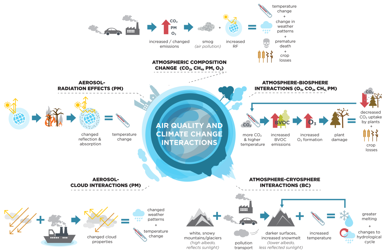
Figure 1. An overview of the main categories of air quality and climate change interactions including a depiction of an example interaction or feedback for each category. Depicted emission sources are examples of possible sources but do not encompass all emission sources relevant to the depicted interaction. The most relevant components are listed in the brackets following the category. PM (particulate matter) indicates all aerosol sources, including OA (organic aerosol), BC (black carbon), and \text{SO}_2 ; \text{O}_3 (ozone) includes \text{O}_3 and its precursor compounds, \text{NO}_x , NMVOCs, and \text{CO} .
