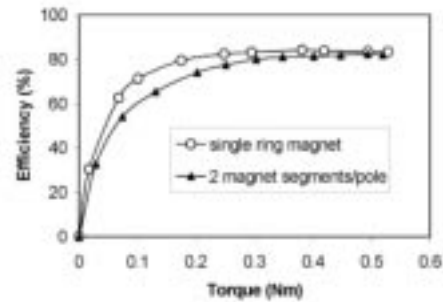
Fig. 8. Measured efficiency–torque characteristics of Halbach magnetized motors.
