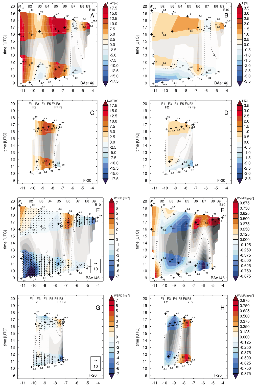
Figure 8. Hovmöller plots showing difference (model minus observations) between BAe146 and F-20 droppsonde measurements (Figure 5) and interpolated Africa-LAM forecasts (Figure 7) of low-level atmospheric thickness defined as the difference between (a and c) 700 and 950 hPa geopotential height, (b and d) air temperature, (e and g) wind speed and direction, and (f and h) water vapor mixing ratio on 22 June 2011. Droppsonde locations are indicated by plus symbols and labeled at the top of each plot. The greyed out contour lines mark the region between the morning and afternoon flights where the temporal interpolation may not be trusted as the time difference is quite large. The dotted line marks the zero line.
