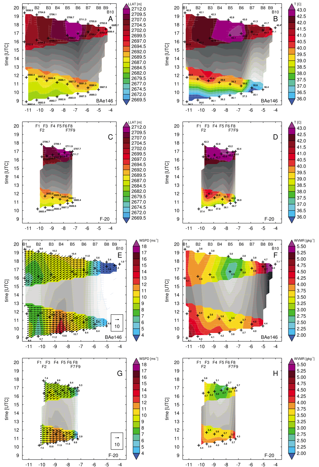
Figure 7. Hovmöller plots (longitude by time) of Africa-LAM forecasts interpolated to BÅe146 and F-20 dropsonde locations and times showing low-level atmospheric thickness defined as the difference between (a and c) 700 and 950 hPa geopotential height, (b and d) 950 hPa air temperature, (e and g) 950 hPa wind speed and direction, and (f and h) 950 hPa water vapor mixing ratio on 22 June 2011. Dropsonde locations are indicated by plus symbols and labeled at the top of each plot. The greyed out contour lines mark the region between the morning and afternoon flights where the temporal interpolation may not be trusted as the time difference is quite large.
