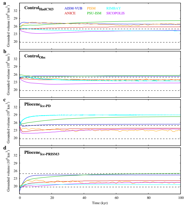
Fig. 2. Modelled grounded ice volume over 100 kyr with Bedmap1. a) The Control HadCM3 simulation, with HadCM3 pre-industrial climate forcing. b) The Control Obs simulation, with ERA-40/WOD09 climate forcing. c) The Pliocene Ice-PD simulation, with HadCM3 Pliocene climate forcing and an initial PD ice sheet. d) The Pliocene Ice-PRISM3 simulation, with HadCM3 Pliocene climate forcing and the initial PRISM3 ice sheet. The horizontal dashed lines indicate the PD and Pliocene grounded ice volume of the Bedmap1 ice-sheet topographies.
