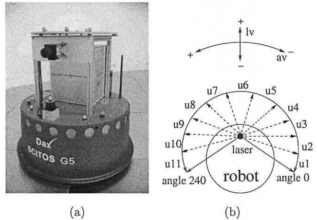
Fig. 5. (a) THE SCITOS G5 ROBOT DAX. DAX HAS TWO DEGREES OF FREEDOM (TRANSLATIONAL AND ROTATIONAL) AND IS A HOKUYO LASER RANGE FINDER. THE RANGE FINDER HAS A WIDE ANGULAR RANGE ( 240^\circ ) WITH A RADIAL RESOLUTION OF 0.36^\circ AND DISTANCE RESOLUTION OF LESS THAN 1CM. (B) IN ORDER TO DECREASE THE DIMENSIONALITY OF THE INPUT SPACE TO THE NARMAX MODEL, WE COARSE CODED THE LASER READINGS INTO 11 SECTORS ( u_1 TO u_{11} ) BY AVERAGING 62 READINGS FOR EACH 22^\circ INTERVALS.
