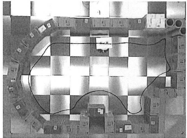
Fig. 3. EXPERIMENT 1: THE TRAJECTORY OF THE ROBOT DRIVEN BY THE ARMAX CONTROLLER GIVEN IN TABLE 1 RESEMBLES THE TRAINING TRAJECTORY (FIGURE 2) VERY CLOSELY.
