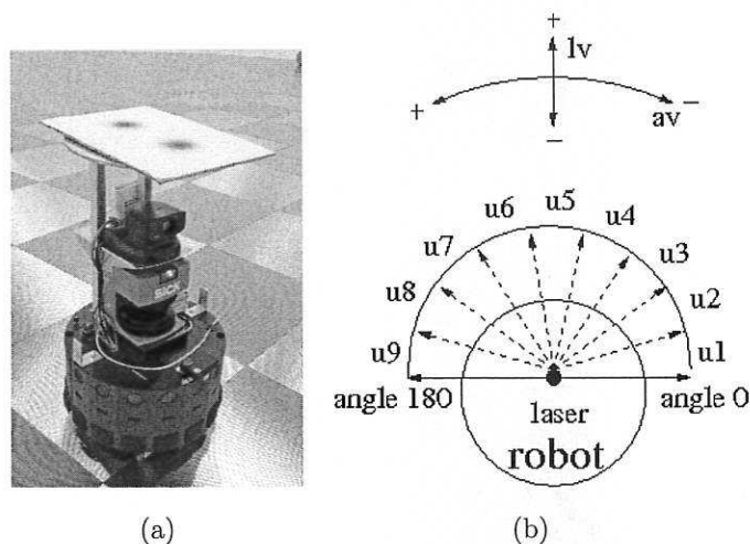
Fig. 1. (A) RADIX HAS TWO DEGREES OF FREEDOM (TRANSLATIONAL AND ROTATIONAL). THE ROBOT IS EQUIPPED WITH A LASER RANGE FINDER, SONAR AND INFRARED SENSORS AS WELL AS A CAMERA. THE RANGE FINDER HAS A WIDE ANGULAR RANGE ( 180^\circ ) WITH A RADIAL RESOLUTION OF 1^\circ AND A DISTANCE RESOLUTION OF LESS THAN 1CM. (B) DURING EXPERIMENTS, IN ORDER TO DECREASE THE DIMENSIONALITY OF THE INPUT SPACE TO NARMAX MODEL, WE COARSE CODED THE LASER READINGS INTO 9 SECTORS ( u_1 TO u_9 ) BY AVERAGING 20 READINGS FOR EACH 20^\circ INTERVALS.
