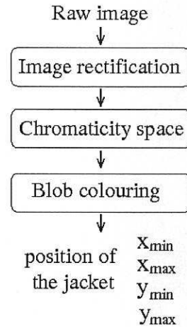
Fig. 11. THE BLOCK DIAGRAM THAT ILLUSTRATES HOW THE POSITION OF THE RED JACKET IS EXTRACTED FROM THE CAPTURED IMAGES. FIRST THE LENS DISTORTIONS ARE REMOVED FROM THE RAW IMAGE. THEN THE CORRECTED IMAGE IS CONVERTED INTO CHROMATICITY SPACE WHICH IS LESS ILLUMINATION DEPENDENT. IN THE FINAL STAGE, THE JACKET IS SEPARATED FROM THE BACKGROUND OF THE IMAGE BY BLOB COLOURING ALGORITHM (SEE FIGURE 10).
