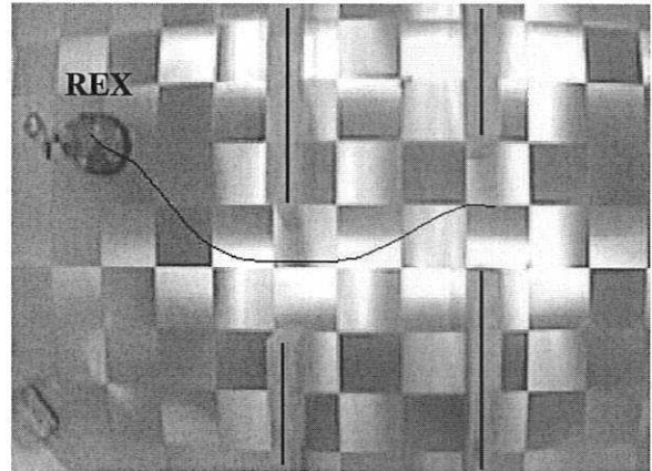
Fig. 18. EXPERIMENT 3: THE TRAJECTORY OF THE ROBOT UNDER THE CONTROL OF THE GIVEN VELOCITY COMMANDS OBTAINED FROM THE HUMAN TRAJECTORY GIVEN IN FIGURE 16, NOT USING ANY SENSORY PERCEPTION. DURING THIS PASS, Rex LOGS ITS OWN PERCEPTION PERCEIVED ALONG THE TRAJECTORY AND THE VELOCITY COMMANDS. THE LOGGED DATA IS THEN USED TO OBTAIN SENSOR-BASED CONTROLLERS WHICH LINK THE PERCEPTION OF THE ROBOT TO THE DESIRED BEHAVIOUR.
