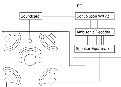
Figure 1: System diagram of a typical FOA-based real-time auralisation system (only 4 loudspeakers are shown for clarity)
