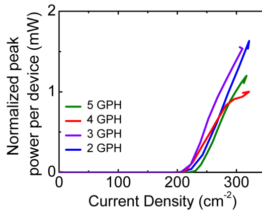
Fig. 7. LI characteristics normalized by the number of devices in the array. The LI characteristics of Fig. 6(d) are presented here normalized by the number of elements in the array. The slope efficiency per unit device in the arrays are the same within \pm 5\% , except for the array of 4 which is under-performing. The exact values are, in \text{mW/kAcm}^{-2} : 17.7 (array of two); 17 (array of 3); 13 (array of 4); 16 (array of 5). This suggests that the performance of each emitting unit in the coupled system is maintained independently of the number of GPH in the array.
