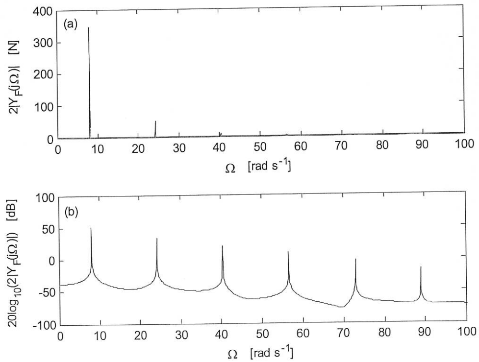
Fig. 4. The output frequency response when f(\bullet) = a_1(\bullet) + a_3(\bullet)^3 , a_1 = 29.6 \text{ s N m}^{-1} and a_3 = 1 \times 10^6 \text{ s N m}^{-1} : (a) Amplitude response, (b) Bode response.
