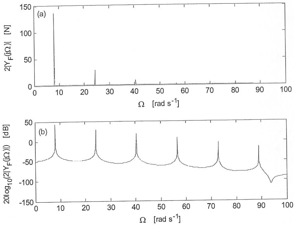
Fig. 4. The output frequency response when f(\bullet) = a_1(\bullet) + a_3(\bullet)^3 , a_1 = 29.6 \text{ s N m}^{-1} and a_3 = 1 \times 10^6 \text{ s N m}^{-1} : (a) Amplitude response, (b) Bode response.
