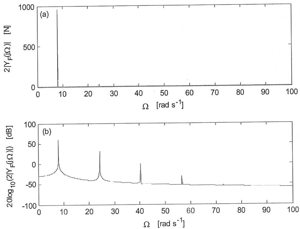
Fig. 3. The output frequency response when f(\bullet) = a_1(\bullet) + a_3(\bullet)^3 , a_1 = 29.6 \text{ s N m}^{-1} and a_3 = 29.6 \text{ s N m}^{-1} .
