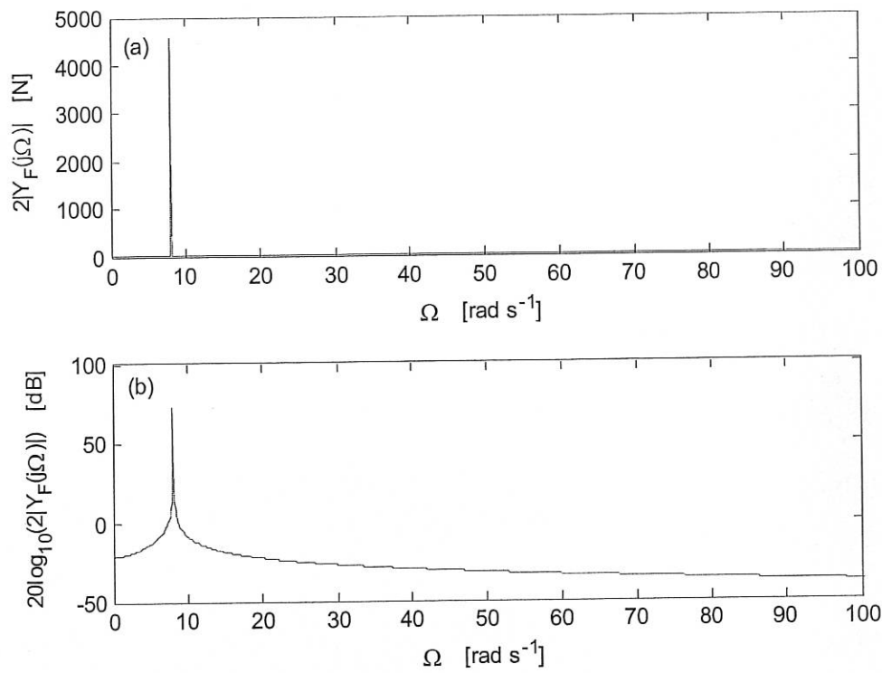
Fig. 2. The output frequency response when f(\bullet) = a_1(\bullet) + a_3(\bullet)^3 , a_1 = 29.6 \text{ s N m}^{-1} and a_3 = 0 \text{ s N m}^{-1} : (a) Amplitude response, (b) Bode response.
