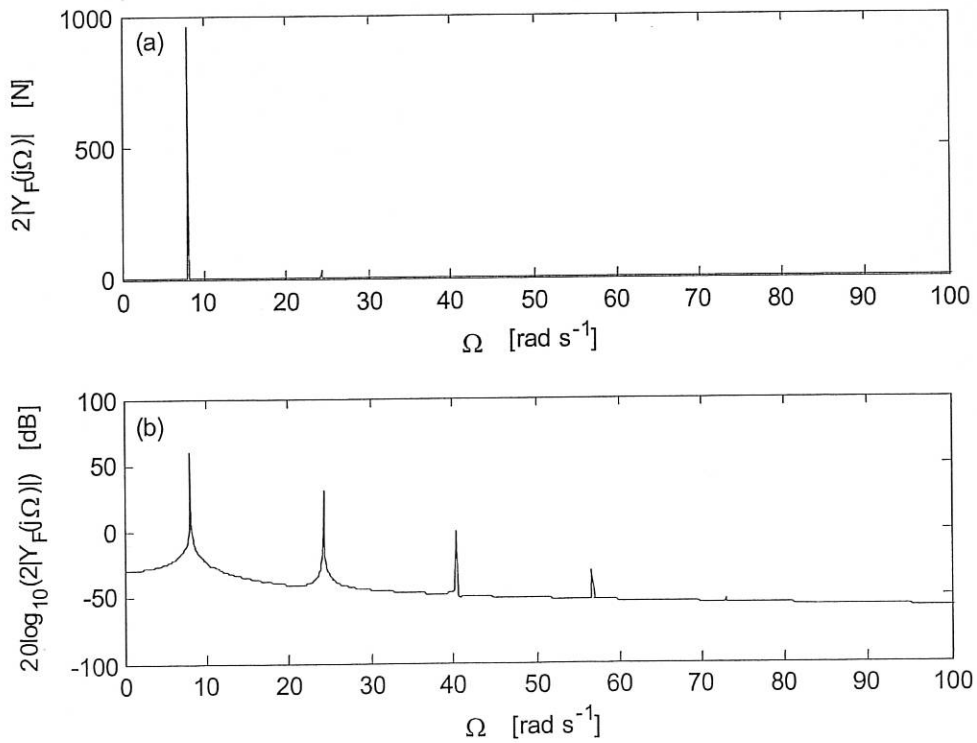
Fig. 3. The output frequency response when f(\bullet) = a_1(\bullet) + a_3(\bullet)^3 , a_1 = 29.6 s N m -1 and a_3 = 29.6 s N m -1 .
