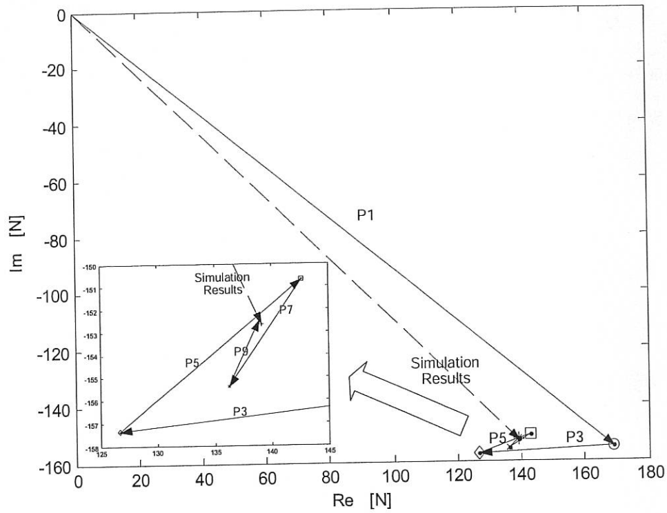
Fig. 10. The output frequency response Y_F(j\Omega) at the driving frequency \Omega when f(\cdot) = a_1(\cdot) + a_3(\cdot)^3 , a_1 = 29.6 \text{ s N m}^{-1} and a_3 = 200 \text{ s N m}^{-1} . Solid lines: analytically determined results using nonlinear terms up to ninth order; dashed lines: simulation results.
