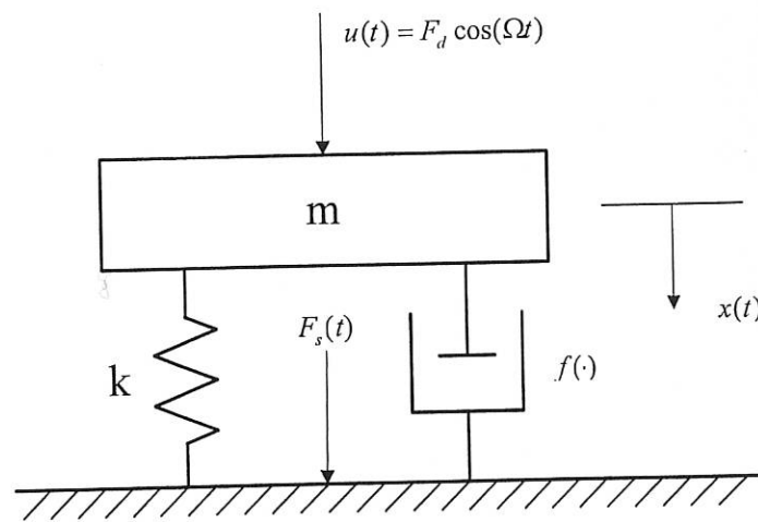
Fig. 1. The SDOF mass-spring-damper system considered in the study
