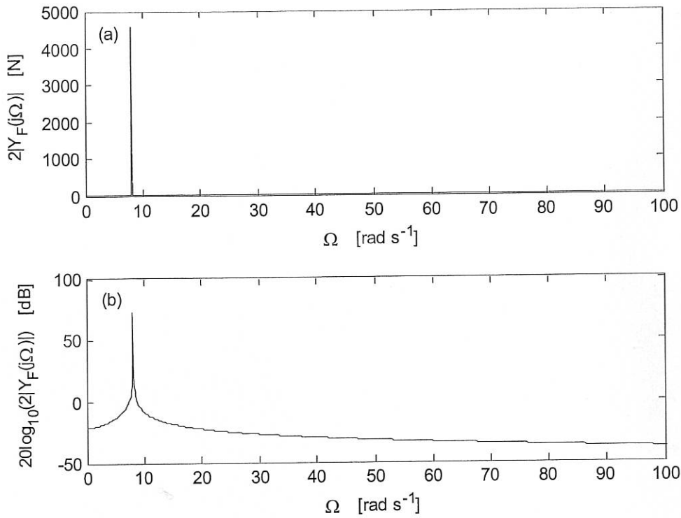
Fig. 2. The output frequency response when f(\bullet) = a_1(\bullet) + a_3(\bullet)^3 , a_1 = 29.6 s N m -1 and a_3 = 0 s N m -1 : (a) Amplitude response, (b) Bode response.
