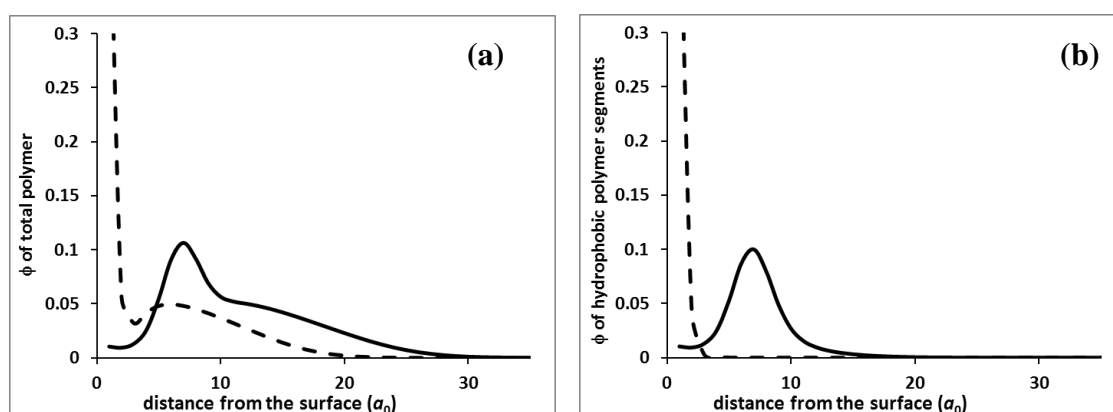
Figure 5. Density profile of biopolymer (a) hydrophobic residues of the biopolymer (b), plotted as a function of distance away from the interface, for the LSC (dashed line) and HSC (solid line) phases.
