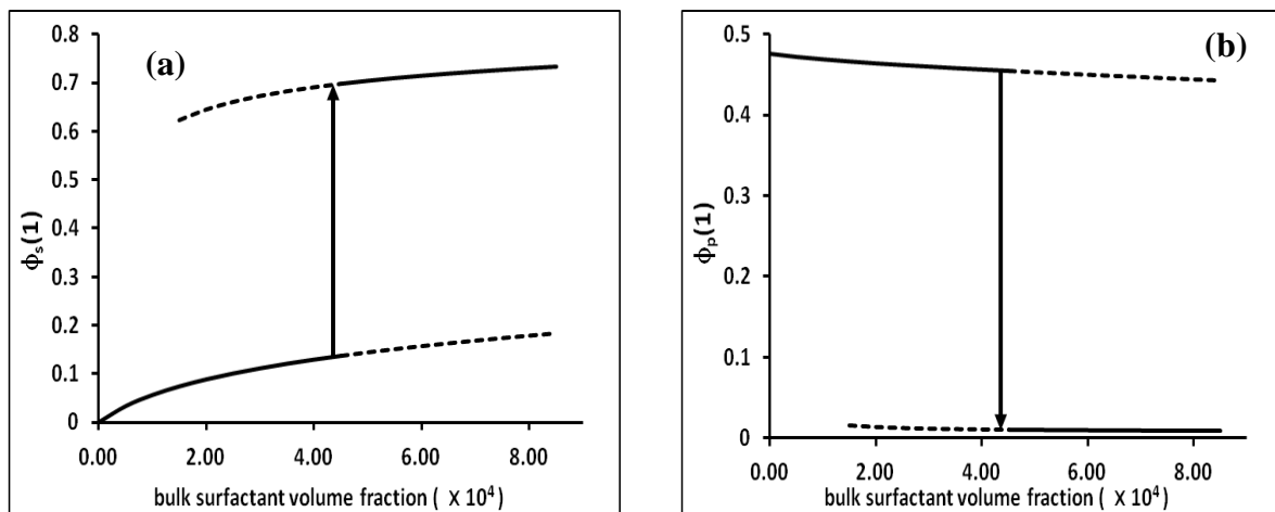
Figure 2. Variation in the number of contacts between the surface and surfactant monomers (a) monomers belonging to chains (b), plotted against the volume fraction of the surfactant in the bulk solution. Dotted lines indicate the values obtained for the metastable states.
