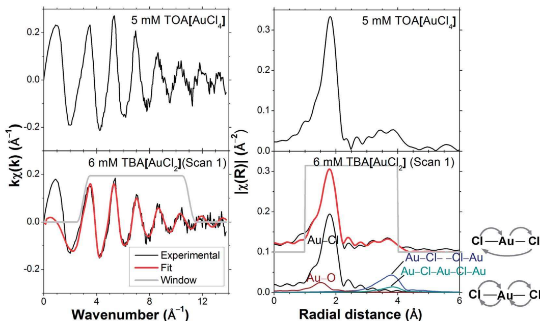
Fig. 2 EXAFS of 6 mM TBA [\text{AuCl}_2] in DCB (sample #1 in Table 1) contrasted with 5 mM TOA [\text{AuCl}_4] in DCB (sample #7). The multiple scattering paths are also shown on the right.
