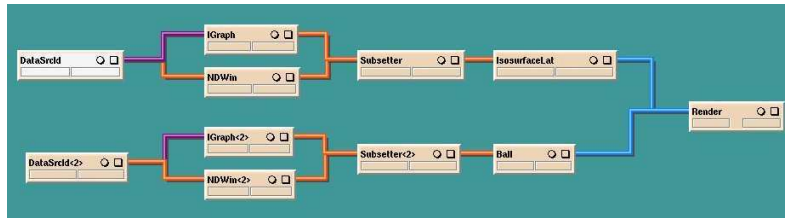
Fig. 10. IRIS Explorer map showing two distinct pipelines, the top one for the multidimensional data (Rosenborck function in 4D) and the bottom one for the multivariate data (the optimization trajectory). Both pipelines make use of the same type of modules for filtering the data. At the end the output of both pipelines are combined into a single visualization.
