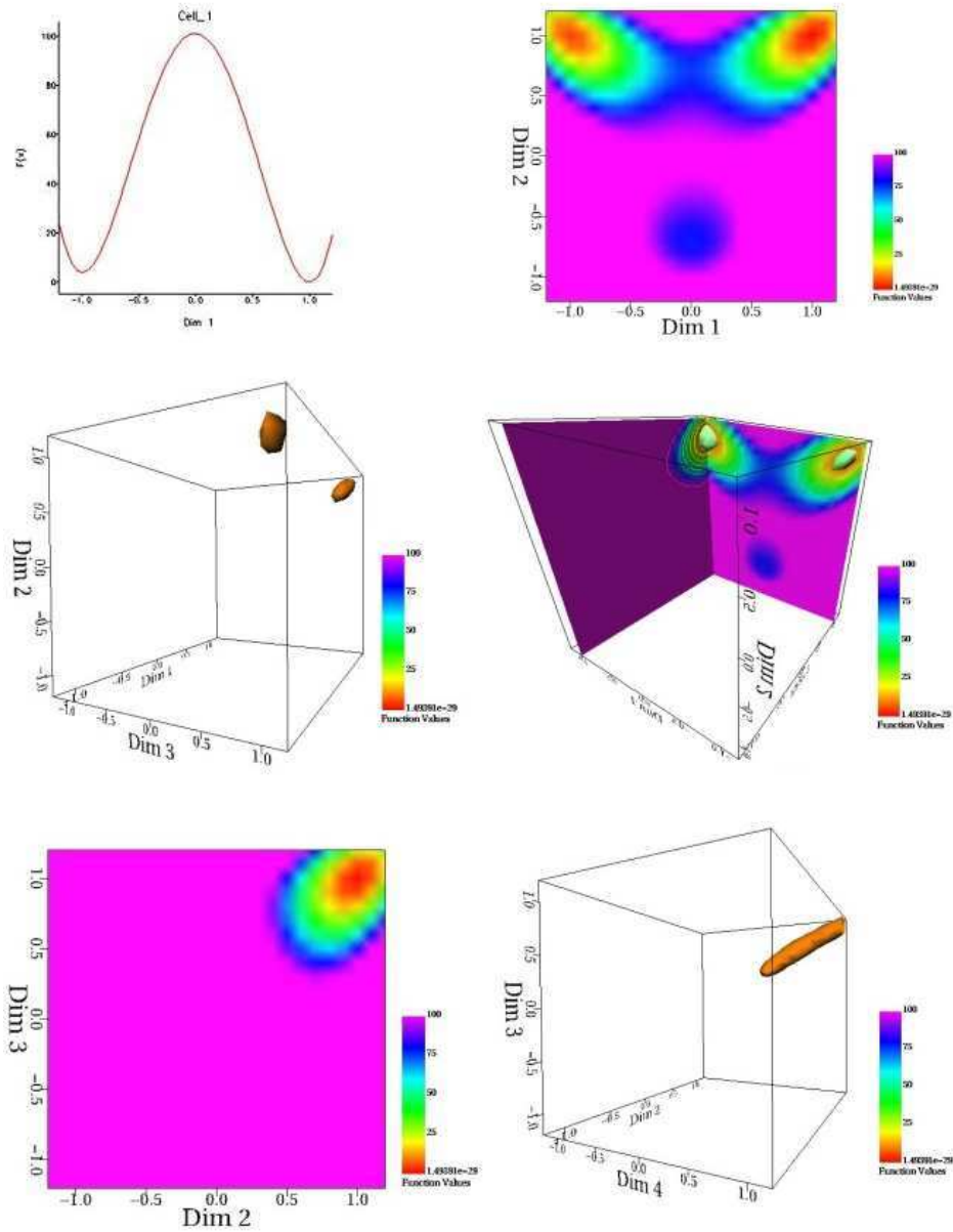
Fig. 9. Progressive exploration of the Rosenbrock function in 4D. These pictures are visualizations with different dimensionality and combination of dimension, taken from the same focus point located at (1,1,1,1). From top to bottom, left to right: Cell-(1), 1D line graph, dimension 1 is free to vary over its range; Cell-(1,2), a 2D coloured map with colours assigned according to the function values, dimensions 1 and 2 are free; Cell-(1,2,3), an isosurface of value 10, dimensions 1, 2 and 3 are free; Cell-(1,2,3), isosurface of value 10, combined with Cell-(1,2) and Cell-(2,3) which are slices of the Cell-(1,2,3); Cell-(2,3), a 2D coloured map, dimensions 2 and 3 are free; Cell-(2,3,4), an isosurface of value 10, dimensions 2, 3 and 4 are free.
