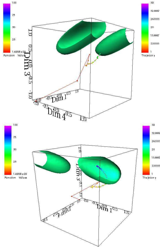
Fig. 12. Further visualization of the 4D Rosenbrock function (multidimensional data) with the successive approximations to the minimum generated by the simplex method (multivariate data). This Figure shows the Cell-(1,3,4) with two regions of low value (contrast with Cell-(2,3,4) in Figure 11 where there is only one region).
