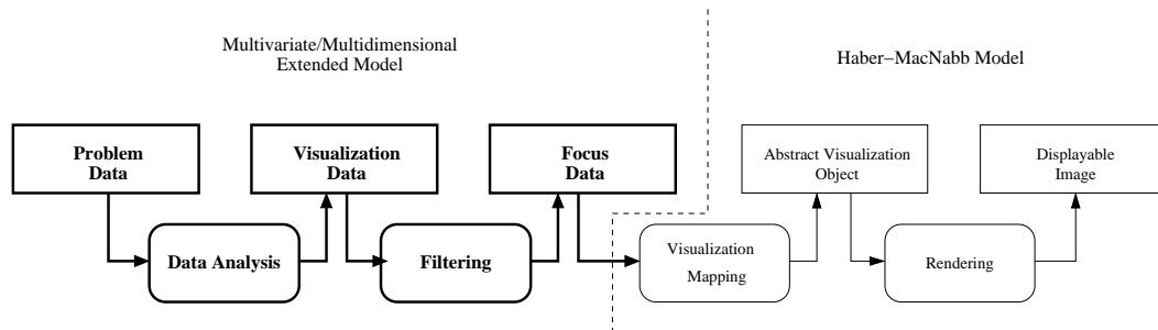
Fig. 1. Haber-McNabb Dataflow Model for Scientific Visualization.
