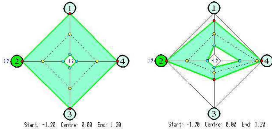
Fig. 4. User interface for the n -dimensional Window definition tool for a 4-dimensional case. The picture on the left shows the starting configuration for the tool, having the range for each dimension (numbered from 1 to 4) set to cover the whole data set. The picture on the right shows the same tool after some interaction has been done, in particular on the ranges of dimensions 1, 3 and 4. Also notice that the focus point (represented by a dashed polyline connecting the yellow circles inside the green region) has also been changed to a different position in the 4-dimensional space. The text at the bottom of each picture shows three numeric values related to the dimension 2, the currently selected dimension (which is indicated by a darker background on the dimension indicator circle): Start , the lower limit for the extent of the domain in that dimension; Centre , the current value for that component of the n -dimensional focus point, and End , the upper limit for the extent of the domain in that dimension. By dragging the corresponding circles the user can change those values.
