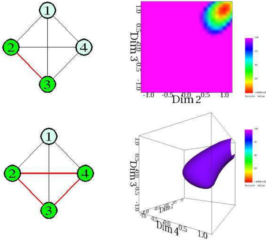
Fig. 6. User interface for the Interaction Graph tool along with several visualizations. The sequence of pictures depicts a further investigation of the 4D space around the focus point, started in Figure 5. The top row corresponds to the Interaction Graph after the dimension 1 has been deselected and a corresponding 2D coloured field generated. The bottom row shows the Interaction Graph after the dimension 4 has been selected, which returns the output to a 3D visualization but now of a different 3D subspace (2-3-4-space).
