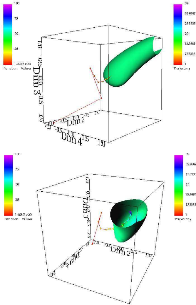
Fig. 11. Combining the visualization of the 4D Rosenbrock function (multidimensional data) with the successive approximations to the minimum generated by the simplex method (multivariate data). Both pictures are of the same subspace Cell-(2,3,4), but taken at distinct viewpoints. The function is represented by an iso-surface of value 50 and the optimization trajectory is represented by a sequence of balls connected by line segments. Each ball represents one step of the optimization algorithm, and its colour is associated with the order of the step in the sequence. Each ball's position in 3D space is obtained by considering only the 2nd, 3rd and 4th coordinates. Note that the last step is at the minimum, located at (1,1,1,1) .
