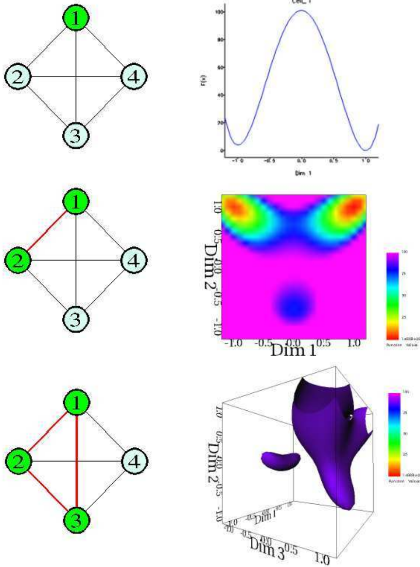
Fig. 5. User interface for the Interaction Graph tool along with several visualizations. The sequence of pictures depicts the action of progressively investigating the 4D space. The left column contains a sequence of Interaction Graphs at different stages of the investigation process. The right column contains the corresponding data visualizations. The top row shows the Interaction Graph with only one dimension selected (dimension 1) and a line graph corresponding to the visualization of the data having that dimension free to vary over its range and the other three dimensions fixed to the values of the focus point. The middle row indicates that the user has selected a second dimension (dimension 2) and the visualization has been changed from the 1D line-graph to a 2D coloured field. In this case the dimensions 1 and 2 are free and dimensions 3 and 4 are the values of the focus point. The bottom row shows that currently 3 dimensions have been selected and a typical 3D visualization method, namely isosurfacing, has been applied to the 3D output data.
