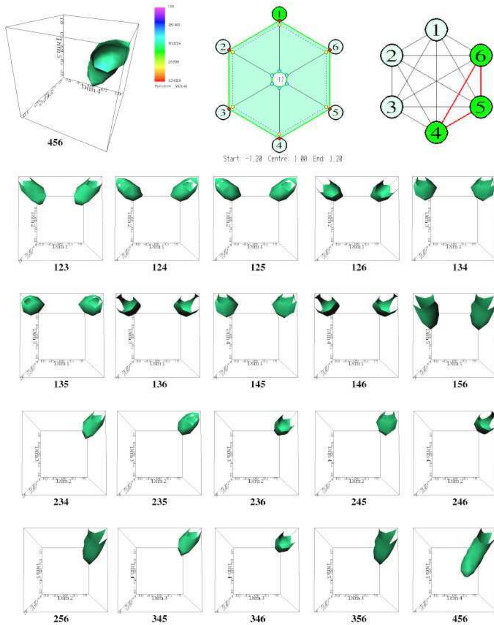
Fig. 14. Showing a visualization of the 6D Rosenbrock function (multidimensional data) through all possible combinations of 3 dimensions, making a total of twenty distinct 3D subspaces. The three pictures on the top, starting from left are: visualization of a chosen subspaces, Cell-(4,5,6); the n -dimensional Window definition tool set for the 6-dimensional case; and the corresponding Interaction Graph having the dimensions 4, 5 and 6 selected. Just below them we have all the subspaces in a subsampled version to allow an overall view of the function. All the subspaces are obtained using the focus point (1,1,1,1,1,1).
