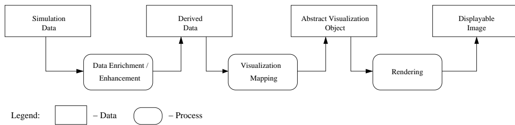
Fig. 1. Haber-McNabb Dataflow Model for Scientific Visualization.
