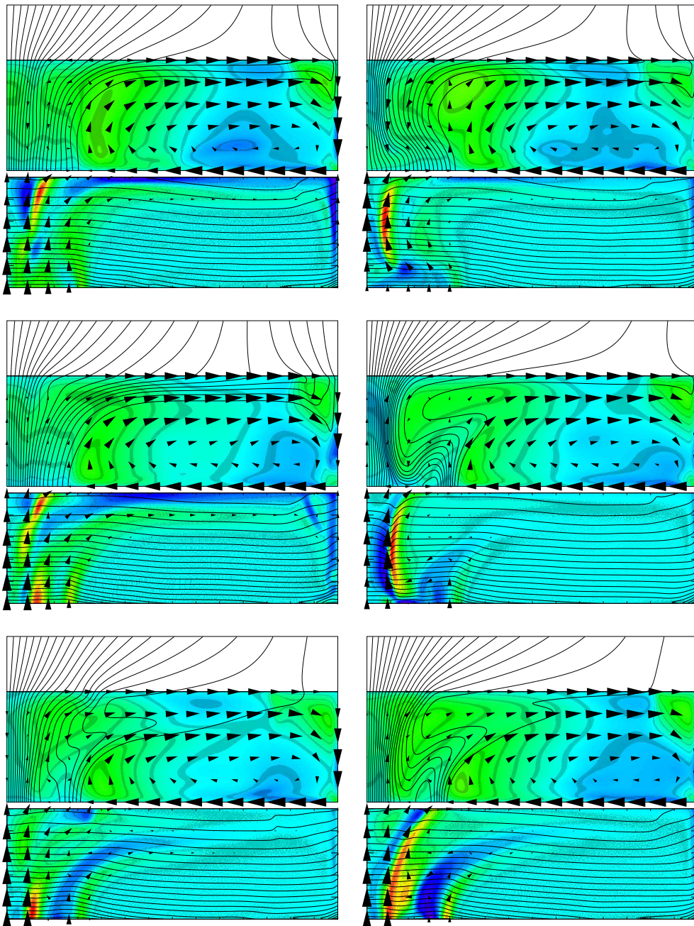
Figure 1: The six 2D plots show a time sequence in the clockwise direction, which is the same direction as movement in the main convection cell. Each plot consists of three boxes in the (r, z) plane. The top (black and white) box is the potential field. The middle box shows the magnetic field lines as contours, the temperature in colour and the velocity as arrows. The bottom box shows the magnetic field strength as arrows, the density as contour lines and the current in the \phi direction in colour. These results were obtained with parameter values R = 10^6 , Q = 100 , \sigma = 0.1 , \zeta_0 = 0.2 , m = 1.45 , and K = 0.529 .
