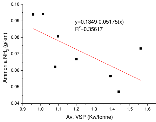
Figure 38: Trip mean NH 3 emissions Vs vehicle's average trip vehicle specific power
