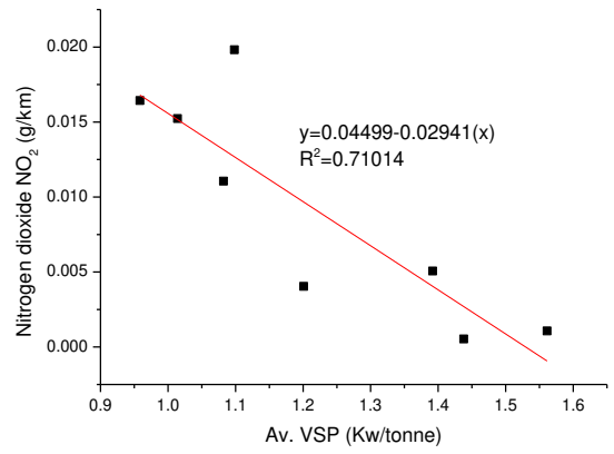
Figure 40: Trip mean NO 2 emissions Vs vehicle's average trip vehicle specific power
