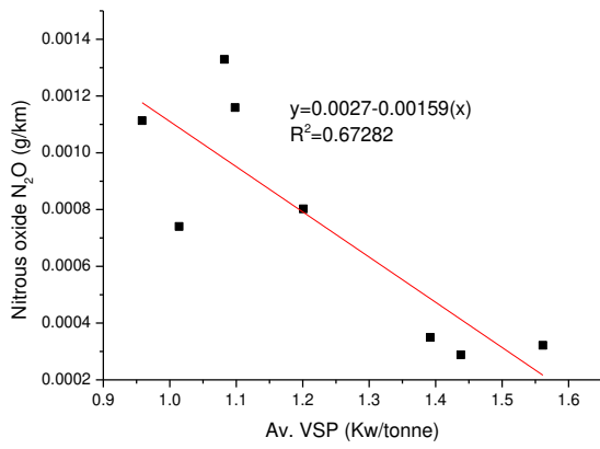
Figure 39: Trip mean N 2 O emissions Vs vehicle's average trip vehicle specific power
