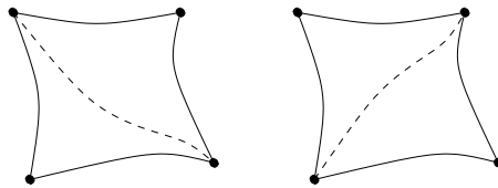
FIGURE 30. Flip of a triangulation.
