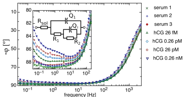
Fig. 3 Typical Impedance phase ( \phi ) spectra recorded by means of EIS (symbols) for successive non-spiked serum injections and increasing concentration of hCG between 26 fM and 0.26 nM in serum. Each spectrum was obtained after 20 minutes of incubation. Lines represent fits to EIS measurements according to the equivalent circuit presented in the inset.
