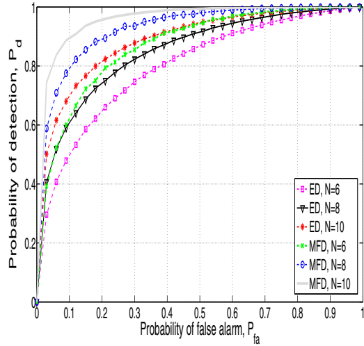
Fig. 4. Probability of detection ( P_d ) versus probability of false alarm ( P_{fa} ), with U = 3 , \xi_a = -4 dB, P_t = 1 and M = 10 .
