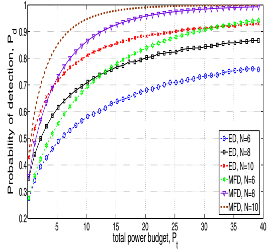
Fig. 5. Probability of detection ( P_d ) versus total power budget ( P_t ), with U = 3 , \xi_a = -4 dB, P_{fa} = 0.1 and M = 20 .
