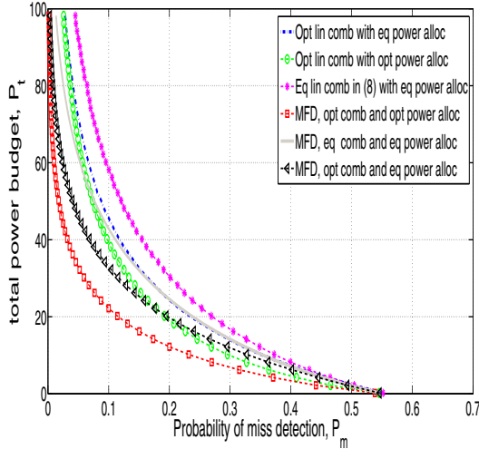
Fig. 3. Total power budget ( P_t ) versus probability of miss-detection ( 1 - P_d ), with P_{fa} = 0.1 , U = 3 , \xi_a = -4 dB, N = 5 and M = 100 .
