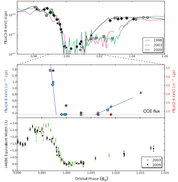
Fig. 2.— Top : X-ray fluxes (3–8 keV) of the CPS (WWC + CCE) measured with Chandra (circle), XMM-Newton (square), Suzaku (triangle), Swift (diamond) and RXTE (solid lines). The red, green and black colors represent measurements around the 1998.0, 2003.5 and 2009.0 minima, respectively. The filled black circles are observed with the Chandra ACIS-S in imaging mode, while the other circles represent ACIS+HETGS grating observations. The sky background in the RXTE light curve ( \sim 3 \times 10^{-11} ergs \text{cm}^{-2} \text{s}^{-1} ) is estimated based on the Chandra observations during the deep minimum (see Section 3) and subtracted from the RXTE light curve. Contribution of the HN emission is also estimated and subtracted from the XMM-Newton , Suzaku and Swift data points. Middle : Soft (2–4 keV, red) and hard (4–8 keV, blue) band fluxes of the CPS during the 2009.0 X-ray minimum. The dotted line is the CCE flux level in both the soft and hard energy bands. The solid lines show linear extrapolations of 4 hard band data points (1 Swift measurement is above this plot) before the ingress and 3 hard band data points after the egress. Bottom : Variation of the equivalent width of the HeII \lambda 4686 line (Teodoro et al. 2012). The color code is the same as in the top panel.
