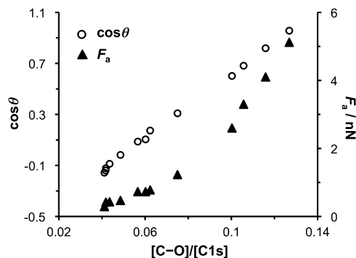
Figure 6. Variation in \cos \theta and F_a with the composition of HUT samples exposed to UV light for varying periods of time and immersed in a solution of DDT.
