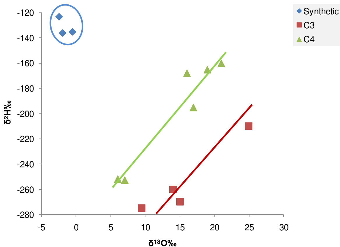
Figure 3.11 The comparison of stable isotope ratios of hydrogen and oxygen for ethanol samples of different origins. The diagram is a simplification of an equivalent graph presented elsewhere [Ishida-Fujii 2005].
