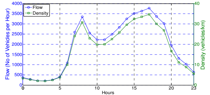
Fig. 2: Hourly Vehicular Flow and Density.
