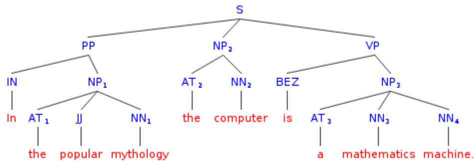
Figure 1: phpSyntaxTree is a web application available under GNU General Public License from sourceforge.net. One departure from convention in this parse tree is the use of Brown POS tags to identify parts of speech at terminal nodes. http://sourceforge.net/projects/phpsyntaxtree
