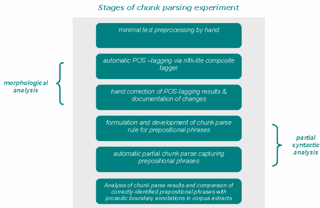
Figure 2: Experimental stages in semi-automatic POS tagging and partial chunk parsing of input text using nltk_lite .
