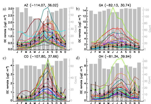
Figure 17. Same as in Fig. 16, for remote stations. Arizona ( a ): 114.07^{\circ} W, 36.02^{\circ} N, years 2000–2006); Georgia ( b ): 82.13^{\circ} W, 30.74^{\circ} N, years 1993–2006); Colorado ( c ): 107.80^{\circ} W, 37.66^{\circ} N, years 2000–2006); Ohio ( d ): 81.34^{\circ} W, 39.94^{\circ} N, years 1998–2004).
