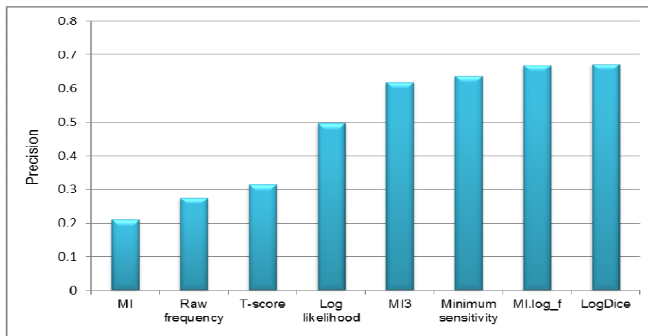
FIGURE 8: Precision scores for the co-occurrence extraction phase.
