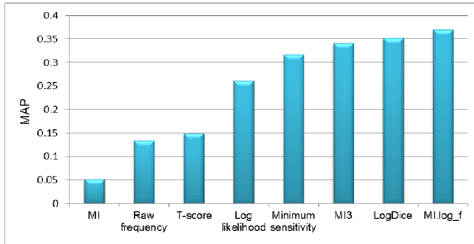
FIGURE 5: MAP scores for the collocation extraction phase.
