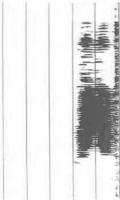
Spectrogram of /tāha/ showing separation of F1 and F2.
