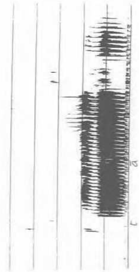
Spectrogram of /tāhin/ showing approximation of F1 and F2.
