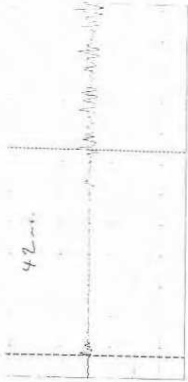
Speech waveform for /t/; left cursor marks release burst, right cursor marks voice onset.
