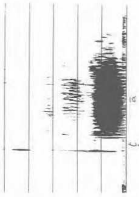
Spectrogram of /tāhin/ showing approximation of F1 and F2.
