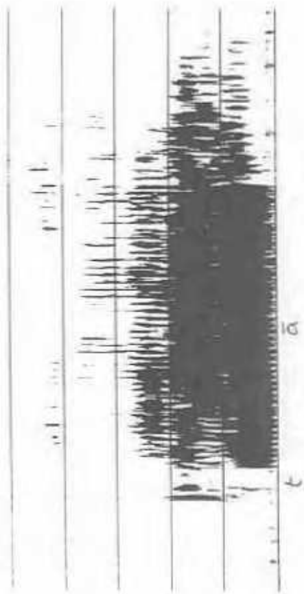
Spectrogram of /taha/ showing separation of F1 and F2.
