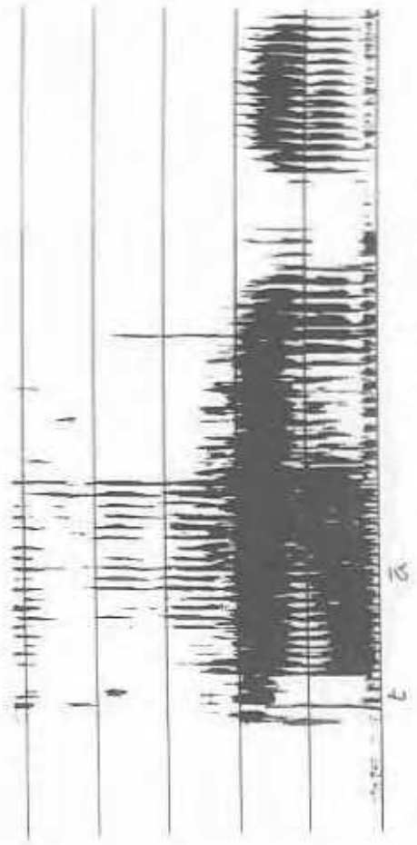
Spectrogram of /tāha/ showing separation of F1 and F2.
