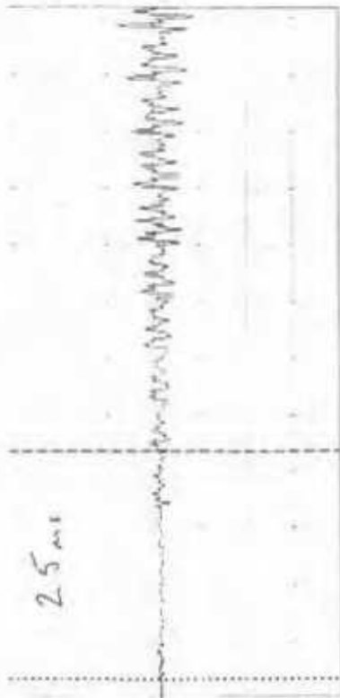
LM (Baghdād) : Speech waveform for /t/; left cursor marks release burst, right cursor marks voice onset.
