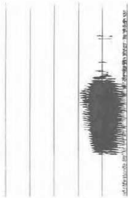
Spectrogram of /tāhin/ showing approximation of F1 and F2.
