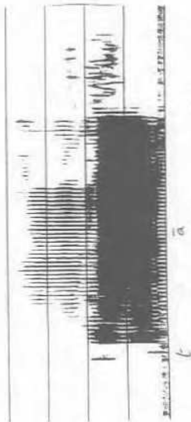
Spectrogram of /tāha/ showing separation of F1 and F2.
