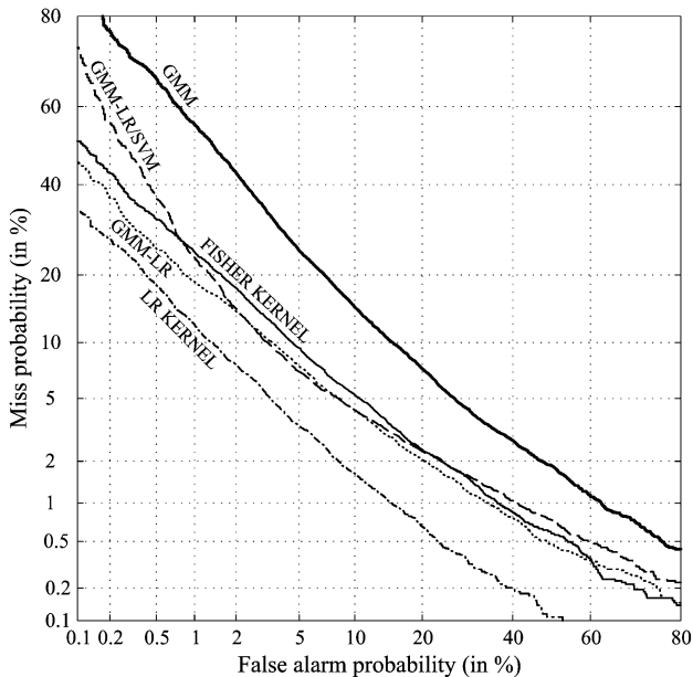
Fig. 3. DET curves of the GMM, GMM-LR, GMM-LR/SVM, Fisher kernel SVM and spherically normalized LR kernel SVM systems for text-independent speaker verification on PolyVar.
