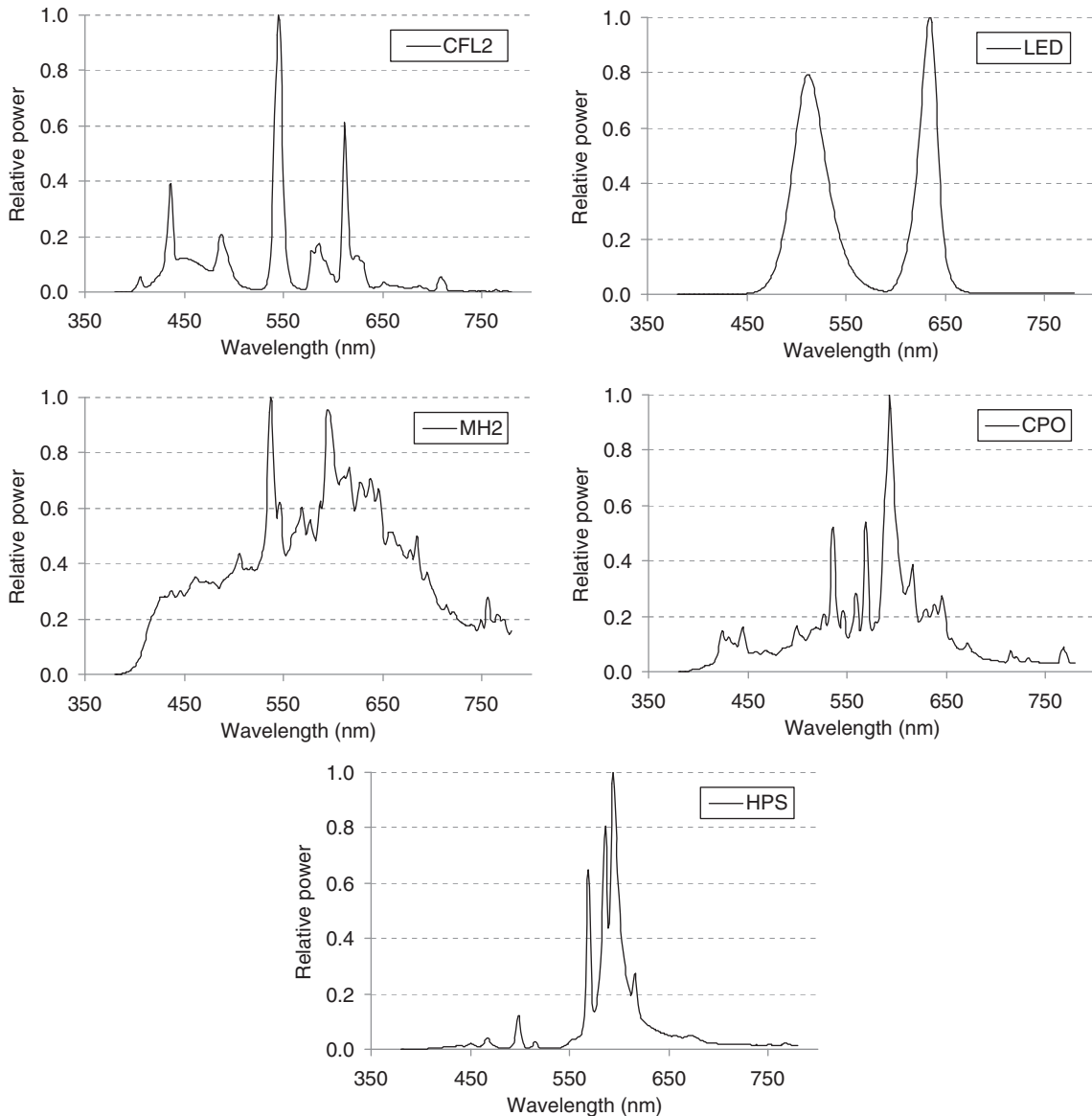
Figure 2 SPDs of the test lamps. These are as measured from the observer's view point and hence include modifications by the test apparatus, and are normalised for a peak response of 1.0
