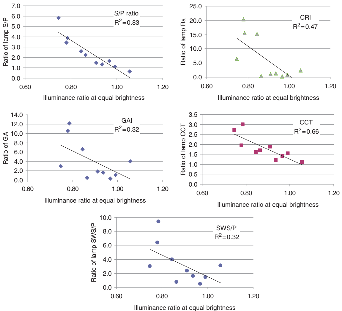
Figure 3 Test results (mean illuminance ratios at equal brightness) plotted against brightness predictions (ratios of lamp characteristics)
