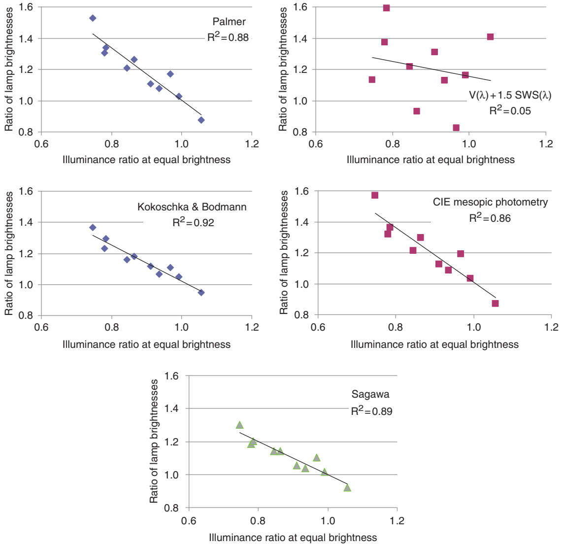
Figure 4 Test results (mean illuminance ratios at equal brightness) plotted against brightness predictions (ratios of brightness model outputs)
