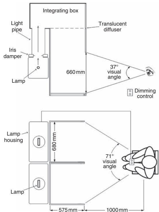
Figure 1 Vertical and horizontal sections through the side-by-side booths used in the brightness ranking and brightness matching tests
