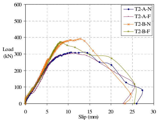
Fig. 10: Load-slip curves of test group T2, tie-bar shear
