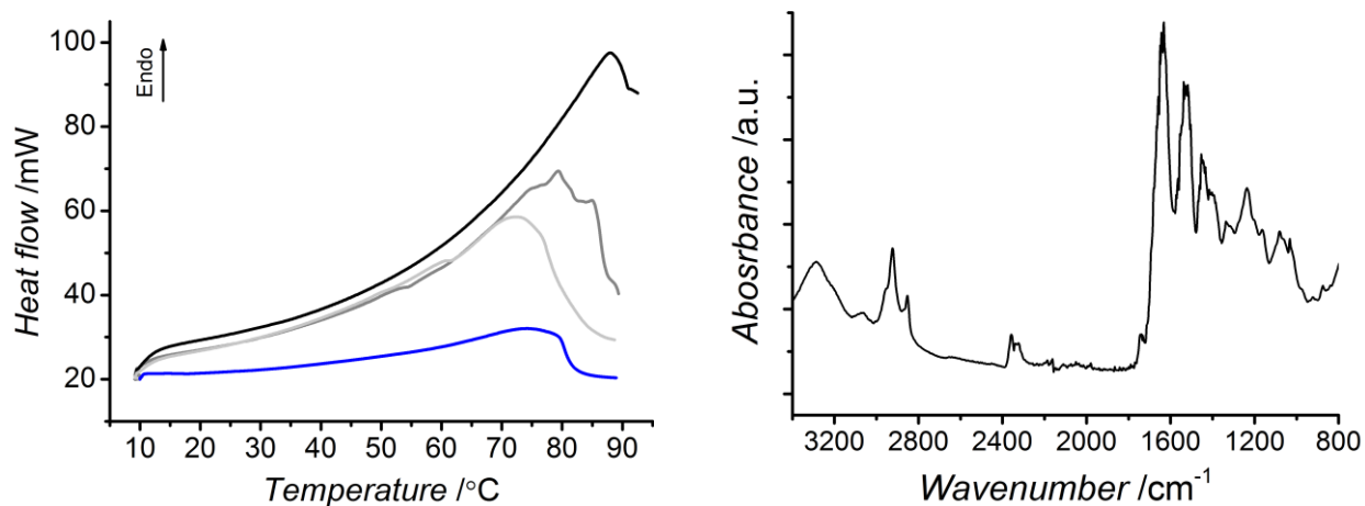
Figure 4. Left: DSC thermograms of samples Collagen-Ph1.5 (—), Collagen-EDC60 (—) and type I collagen (—) obtained with 10 °C·min -1 heating rate. An additional thermogram of sample Collagen-Ph1 was acquired with 1°C·min -1 heating rate (—). All samples describe a triple helix denaturation by an endothermic transition at 67-88 °C. Right: ATR-FTIR spectrum of sample Collagen-Ph1 following DSC analysis; the main peaks of collagen can still be observed in the spectrum.
