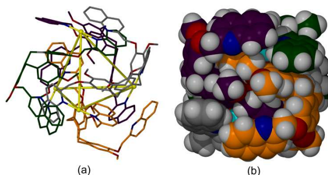
Fig. 3 Crystal structure of the previously reported complex [\text{Ag}_4(\text{L2m})_4]^{4+} , 3m . (a) Highlighting the twisted tetrahedral core, and (b) space-filling diagram displaying the resultant cube-like appearance. 47
