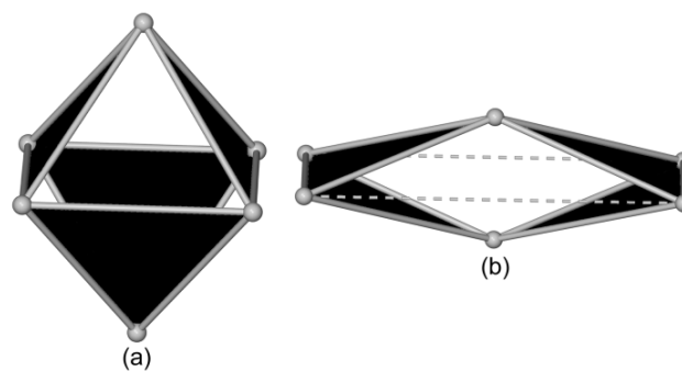
Fig. 6 Comparison of \text{Pd}_6\text{L}_4 assemblies, spheres represent Pd(II) positions taken from crystal structures, while shaded faces show positioning of tripodal ligands. (a) Fujita's octahedral [\text{Pd}_6(\text{en})_6\text{L}_4]^{12+} assembly with vertex sharing L = tris (4-pyridyl)triazine; 54 (b) [\text{Pd}_6(\text{L2p})_4(\text{CF}_3\text{CO}_2)_{12}] assembly with vertex and edge-sharing of ligand positions.
