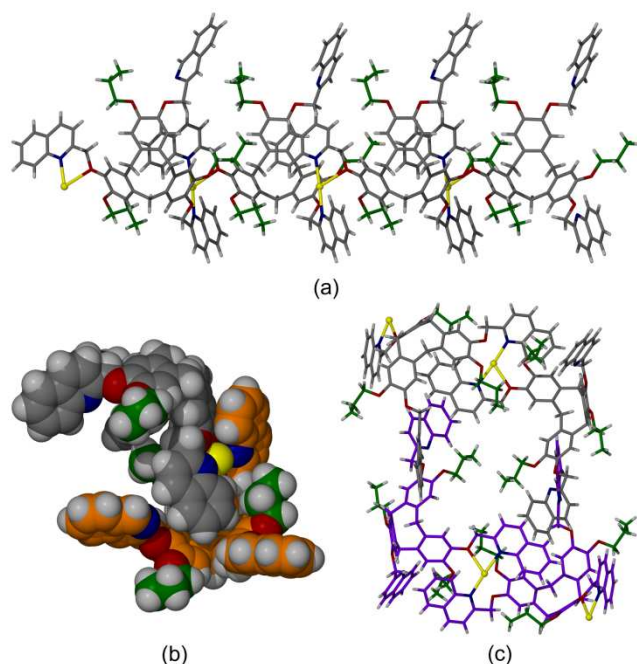
Fig. 4 From the crystal structure of complex 3p . (a) Displaying an individual \{[Ag(L1p)]\}_n 1D polymer unit; (b) Intra-polymer Quinoly-CTG aromatic interactions that are present along the length of individual 1D chains. Independent ligands are colour-coded for clarity; (c) Interstrand aggregation of propyl chains across neighbouring 1D polymers. Individual 1D chains are colour coded, propyl moieties are shown in green and anions and solvent are omitted for clarity.
