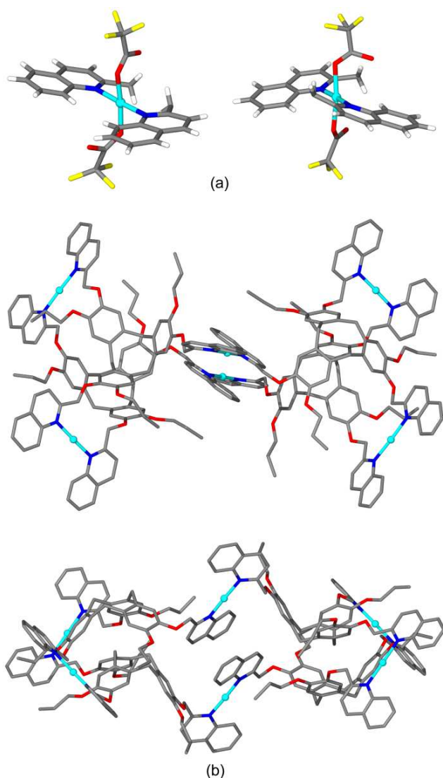
Fig. 5 From the crystal structure of complex 4p (a) The two types of Pd(II) coordination environments showing trans , cis and trans , trans quinolyl arrangements; (b) two views of the of [\text{Pd}_6(\text{L2p})_4]^{12+} assembly, anions are omitted and disordered propyl chains shown in only one position for the sake of clarity.
