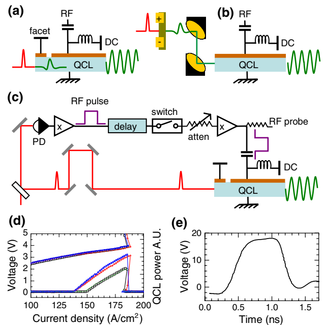
Fig. 1. (Color online) (a) THz pulses are generated inside the QCL by illuminating the seeding section with a fs laser. (b) THz pulses created by an external photoconductive antenna are coupled into a QCL with parabolic mirrors. (c) RF pulses are created with a fast photodiode (PD), and amplified. An electronic delay line is used to vary the RF pulse arrival time. The RF pulse train is modulated with a 50 \Omega switch, and the pulse amplitude can be varied with a variable attenuator. A bias tee allows a quasi-DC voltage to be applied to the QCL along with the RF. A 20 dB pick-off tee (RF probe) allows the RF shape to be monitored. (d) Light-current density ( V - J ) plots for the device with the seeding section biased at 0 V (black), 3.8 V ( \sim 180 A/cm 2 —red), and shorted to the QCL section (blue). (e) RF pulse sent to the QCL measured with the pick-off tee on an 8 GHz sampling oscilloscope (50 \Omega ).
