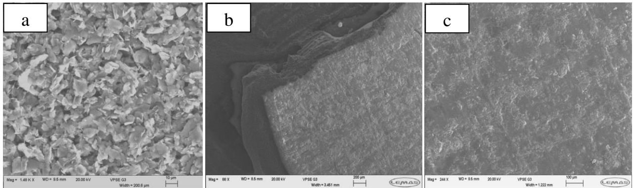
Figure 7. Comparison of densification of a doped CaP pressed pellet with fs-laser (1520 nm) irradiation. a) shows the porous structure before fs-laser sintering; b) after 15 seconds of irradiation, and c) is a high magnification image of area in b) showing evidence for particle densification on a microscopic scale.
