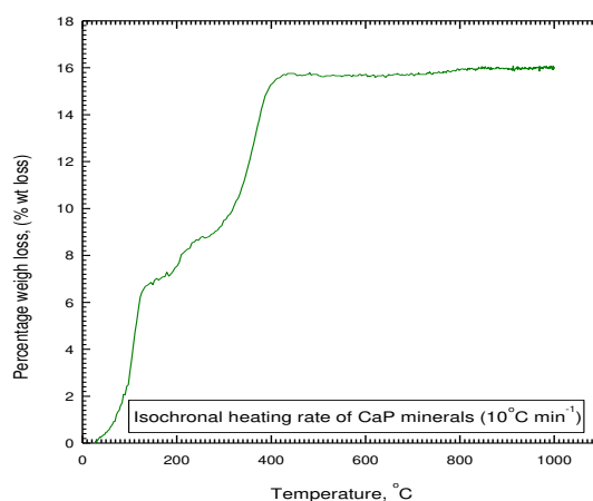
Figure 4. An isochronal heating rate ( 10^{\circ}\text{C min}^{-1} ) weight loss curve for undoped calcium phosphate mineral.
