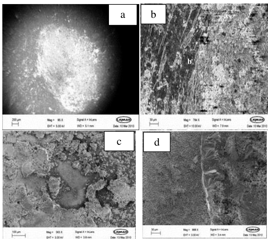
Figure 5. SEM images of (a – b) CaP- \text{Er}_2\text{O}_3 pellet when irradiated with 1520 nm CW laser and (c) \text{Er}_2\text{O}_3 doped CaP coating and, d) CaP- \text{Er}_2\text{O}_3 - \text{AlPO}_4 - \text{CaF}_2 coating over dentine, each of which was irradiated with a 980 nm CW laser for 5 minutes showing the evidence for localized and extensive melting, respectively. Incident laser power was 150 mW at a focus spot.
