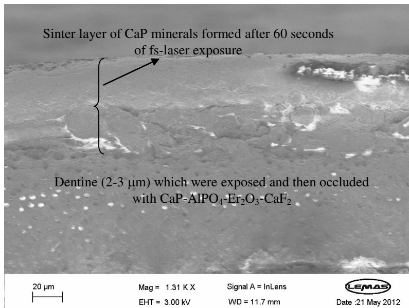
Figure 8. An SEM image of the cross-section of molar, showing dentine tubules which are occluded with a 50 \mu\text{m} thick layer of doped CaP mineral, containing \text{Er}_2\text{O}_3 , \text{AlPO}_4 , and \text{CaF}_2 .
