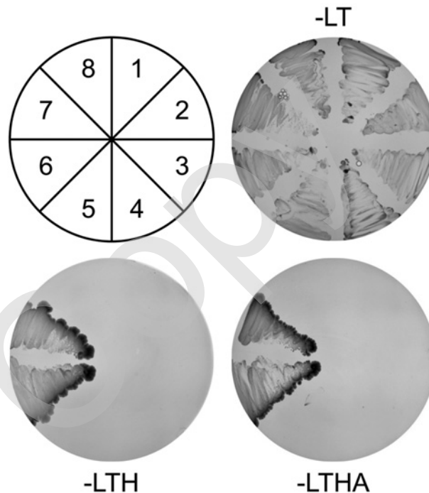
Figure 1 Interaction of the Nac1 and Miz1 POZ domains in yeast two-hybrid assays
