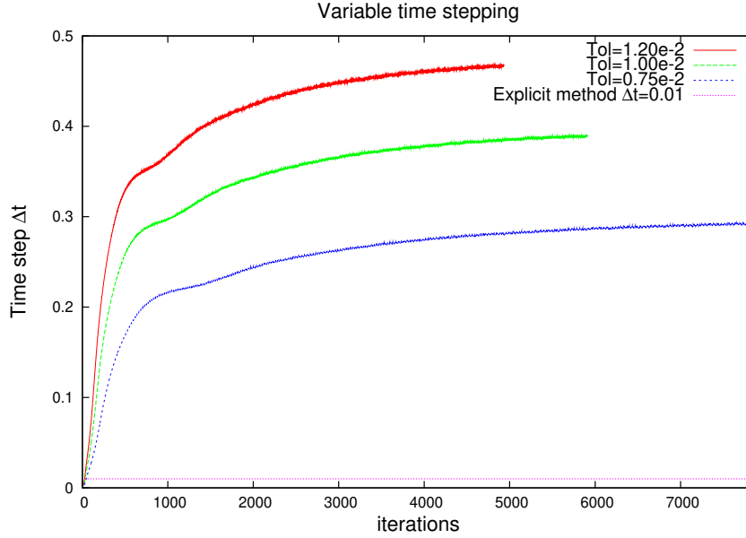
Fig. 4. The evolution of the time step size for t = 0 \dots 2000 , and a minimal element size of h = 0.39 , for different tolerances and in comparison to the constant step size \Delta t = 0.01 for the explicit method
