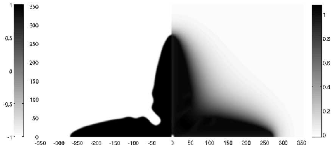
Fig. 6. The interface shape of an alloy dendrite after t = 1800 ; the left and the right box show the contours of the phase variable \phi and the contours of the dimensionless concentration field U , respectively
