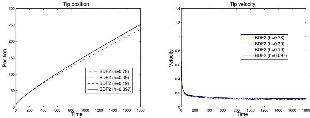
Fig. 11. Convergence study of the dimensionless tip position and tip velocity up to t = 1800 for decreasing element sizes
