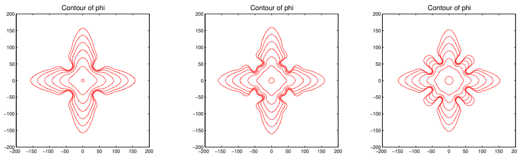
Fig. 7. The evolution of the interface for a different radius of the initial solid seed a) R_0 = 14d_0 b) R_0 = 28d_0 and c) R_0 = 44d_0
