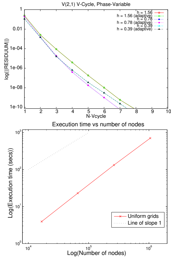
Fig. 5. a)Residual of the phase variable at a fixed time for different mesh levels as well as uniformly and nonuniformly refined meshes; b)shows the execution time for various system sizes
