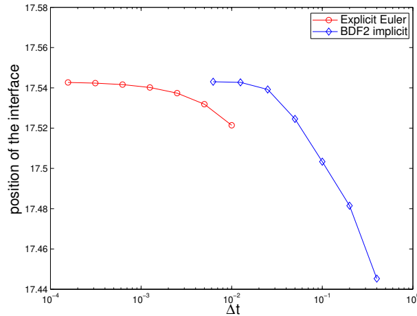
Fig. 3. Convergence study of the position of the interface for different time discretisation methods on uniform grids of element size h = 0.39 and at time t = 10.0 .
