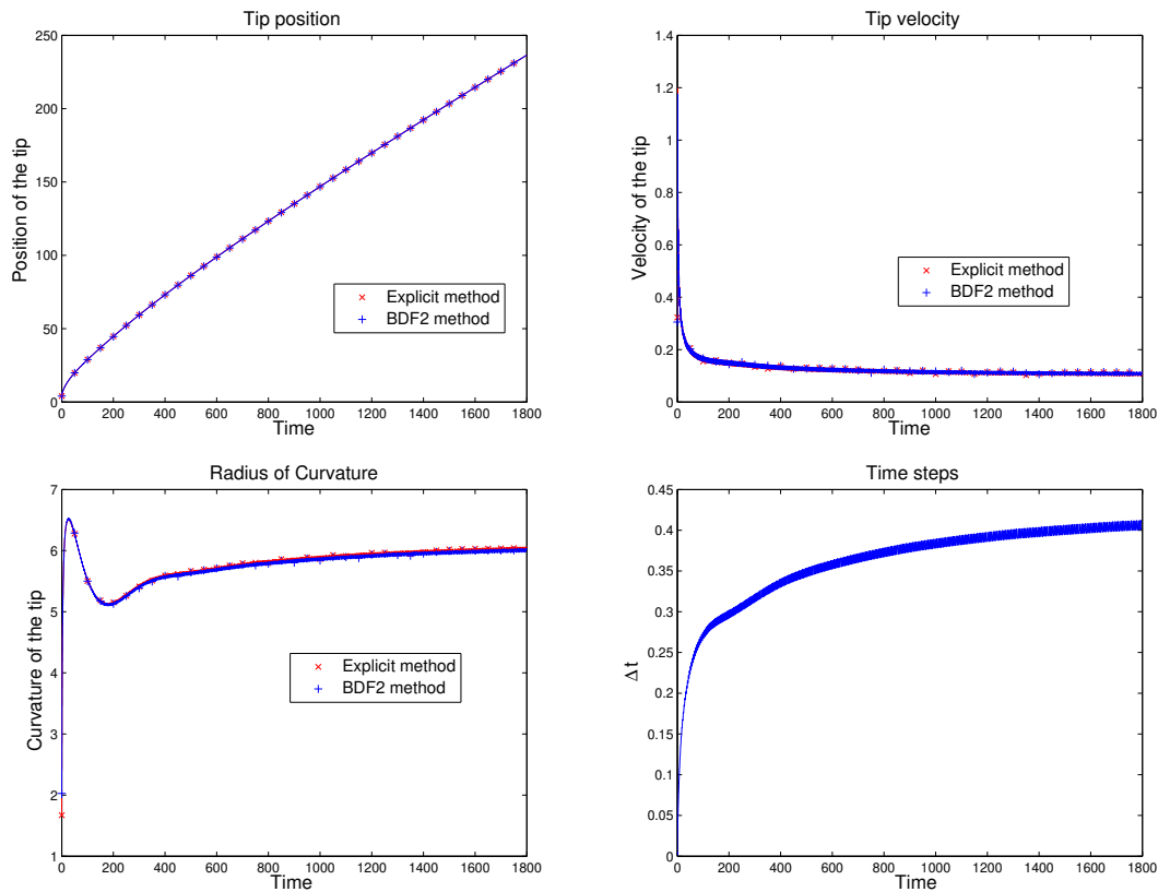
Fig. 9. a)Position of the tip versus time b)Velocity of the tip versus time c)Radius of the tip curvature versus time and d)Evolution of the time steps of the BDF2 method
