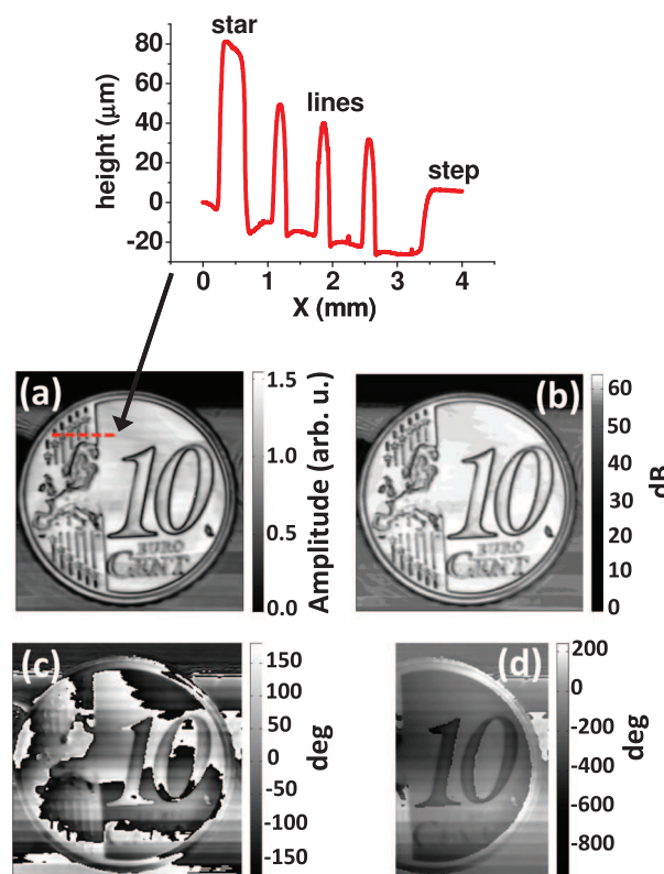
FIG. 3. THz image of a 10 cent Euro coin: (a) amplitude, (b) power, (c) raw phase image, and (d) phase image corrected for the limited phase range of the lock-in amplifier. The coin diameter is 19.75 mm. The image was acquired with lines scans from left to right at a speed of 2.2 \text{ mm/s} , with a step between each line of 100 \mu\text{m} in the vertical direction. The lock-in amplifier time constant was set to 30 ms. Top: height profile obtained by scanning with a profilometer along the red dashed line of (a).
