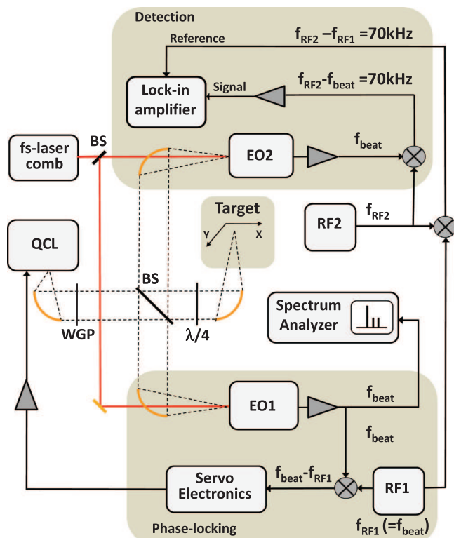
FIG. 1. Experimental apparatus. The fs-laser comb and QCL beams are split into two parts, using two beam splitters (BS), and are focused onto EO detection units EO1 and EO2. EO1 is used to phase-lock f_{\text{beat}} to f_{\text{RF1}} , and therefore to phase-lock \nu_{\text{QCL}} to \sim 10^4 \times f_{\text{rep}} . EO2 is used to detect the THz radiation back-reflected from the imaged target. This is achieved by mixing f_{\text{beat}} ( =f_{\text{RF1}} ) with f_{\text{RF2}} = f_{\text{beat}} + 70 kHz and by monitoring the difference frequency, oscillating at 70 kHz, with a lock-in amplifier. The reference of the lock-in is obtained from the difference frequency f_{\text{RF2}} - f_{\text{RF1}} = 70 kHz. All mirrors used to collimate and focus the radiation from the QCL are 90^\circ off-axis, gold coated parabolic mirrors. The fs-laser comb is a frequency doubled 1550 nm fiber laser emitting a train of \sim 100 fs pulses at a repetition rate f_{\text{rep}} = 250 MHz. There is approximately 15 mW of optical power at 780 nm impinging on each EO detection unit.
