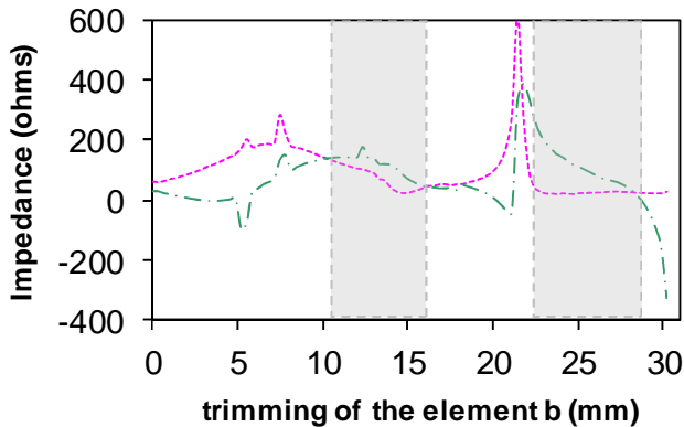
Fig. 4 Tuning of the characteristic impedance of the antenna, real (resistance) and imaginary (reactance) as a function of the trimming of the length of element, b
