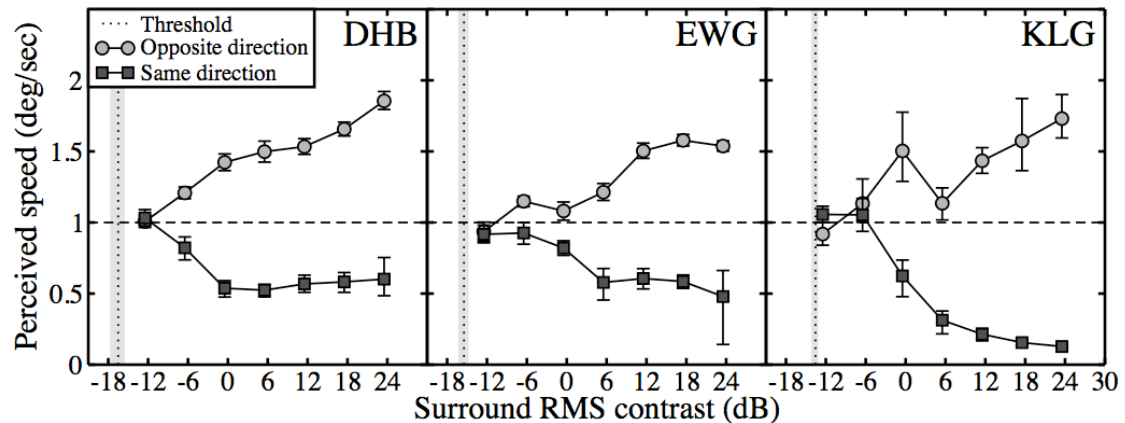
Figure 4: perceived speed as a function of surround contrast. Speed matches are shown for different surround contrasts, and two relative surround directions. The vertical dotted lines are the direction discrimination contrast threshold for the surround noise texture. Grey shaded regions and error bars give 95% confidence limits of threshold and PSE values.
