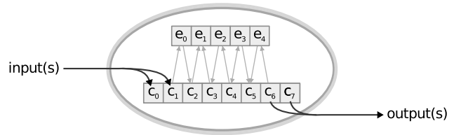
Fig. 4. Artificial metabolic network, where I_C = \{c_0, c_1\} ; O_C = \{c_6, c_7\} .
