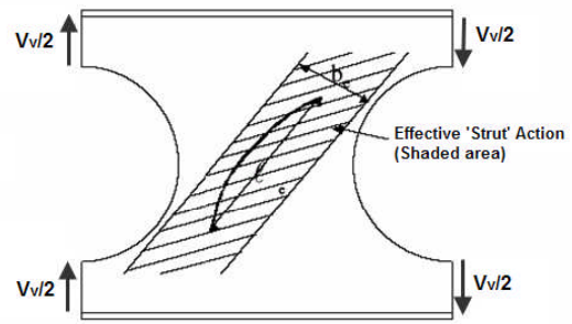
Fig. 8: Strut model of web-post buckling
