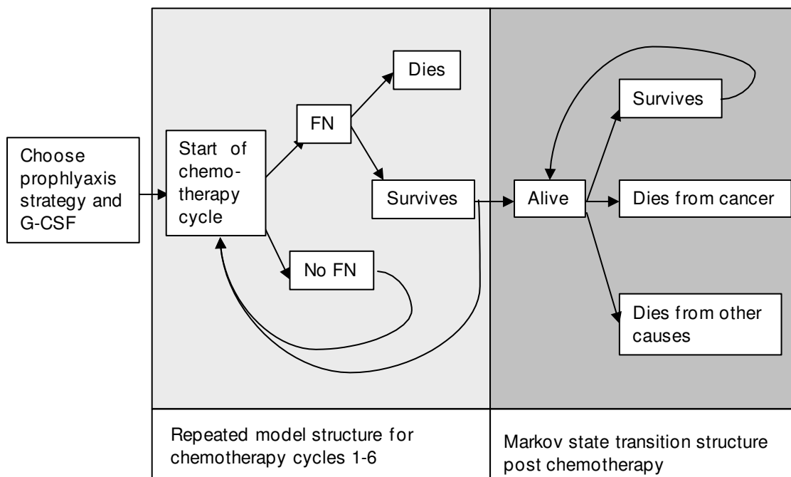
Figure 2: Schematic of the decision analytic model
