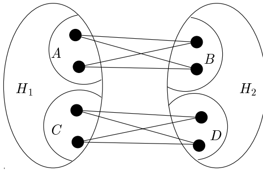
Figure 1: 2-join
